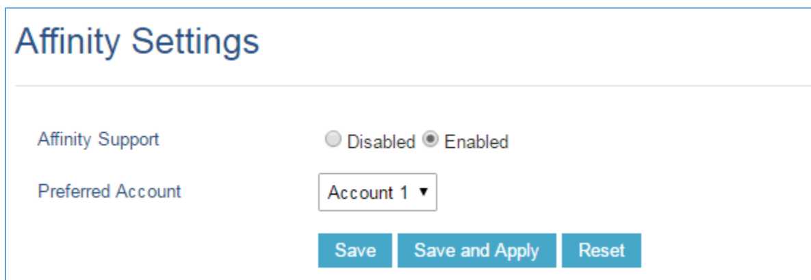
Figure 10: Affinity Settings
