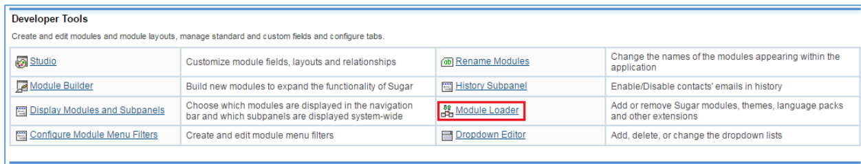
Figure 5: Module Loader
