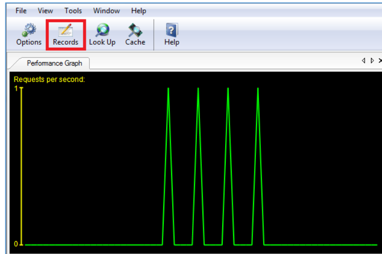
Figure 8: Configure Records
