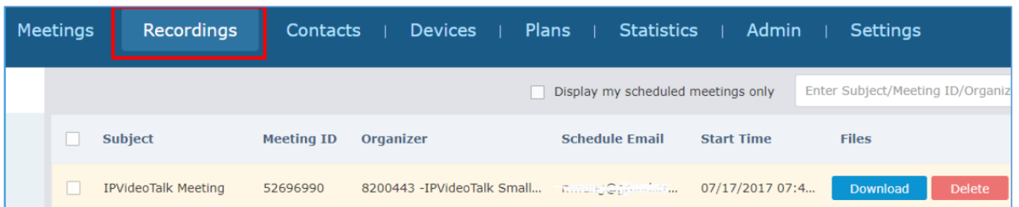
Figure 67 : IPVideoTalk Recordings
