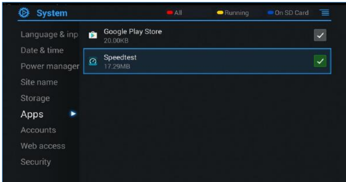
Figure 107: System → Apps
