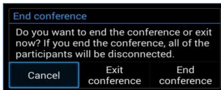
Figure 47: End Conference
