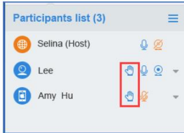
Figure 61: Participants list
