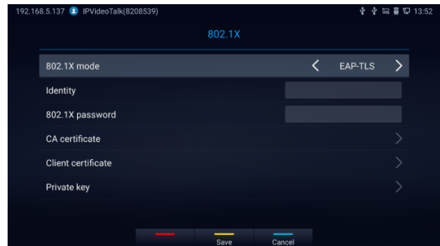
Figure 31: 802.1X - EAP-TLS
