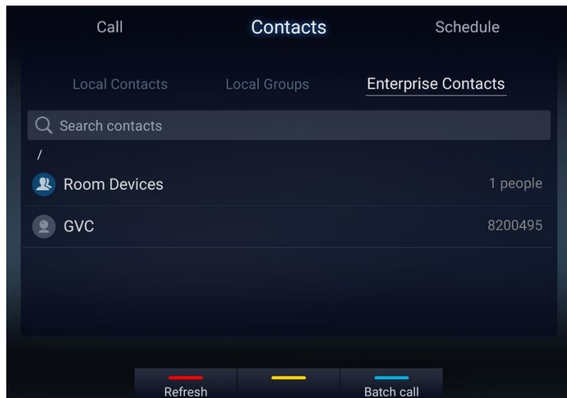
Figure 145: IPVideoTalk - Contacts
