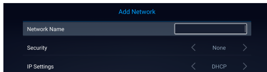
Figure 26: Add Network
