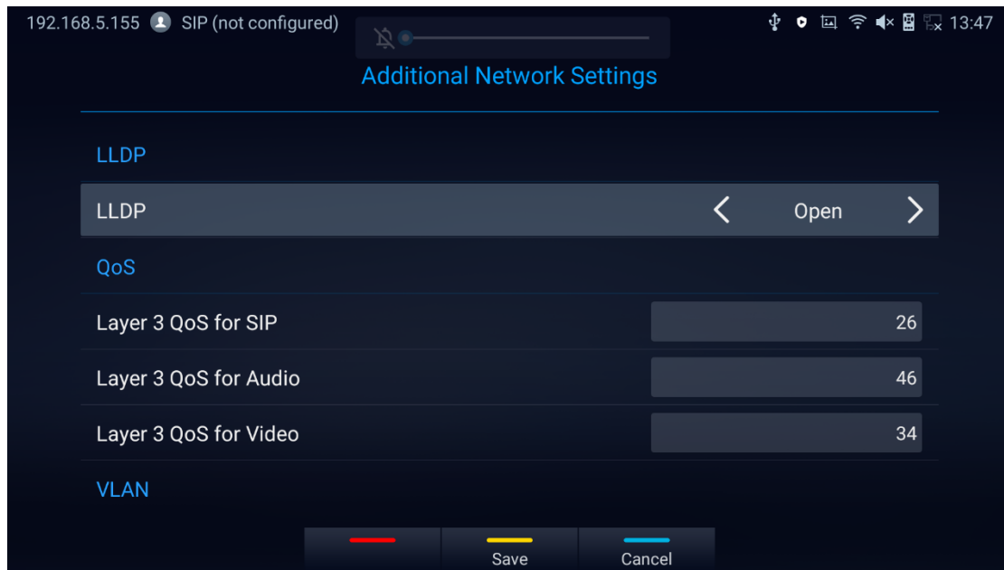
Figure 28: LLDP/VLAN Settings
