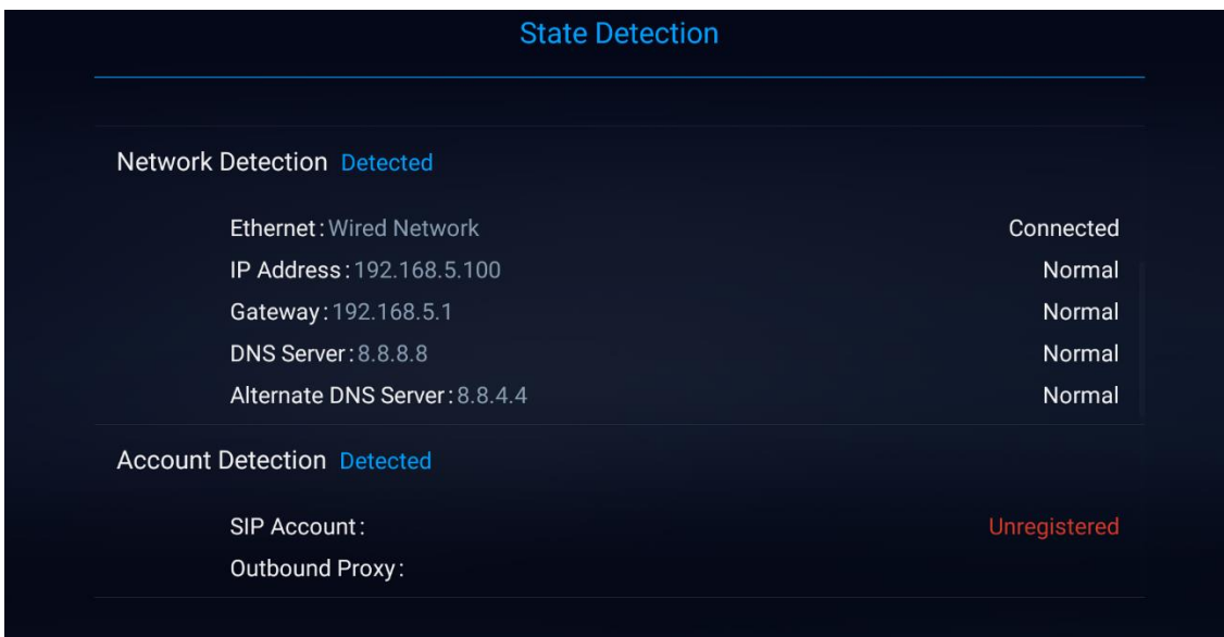
Figure 137: Network/Account Detection
