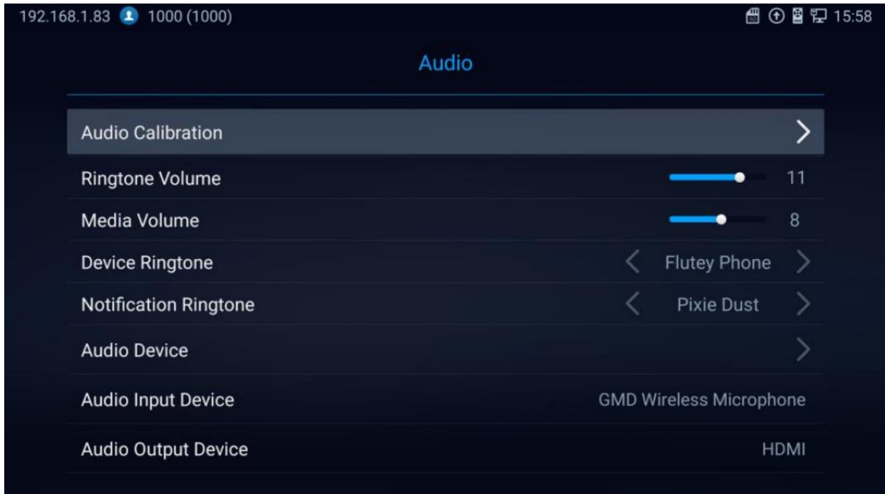
Figure 40: Audio Calibration
