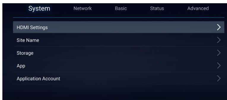
Figure 12: Settings – System
