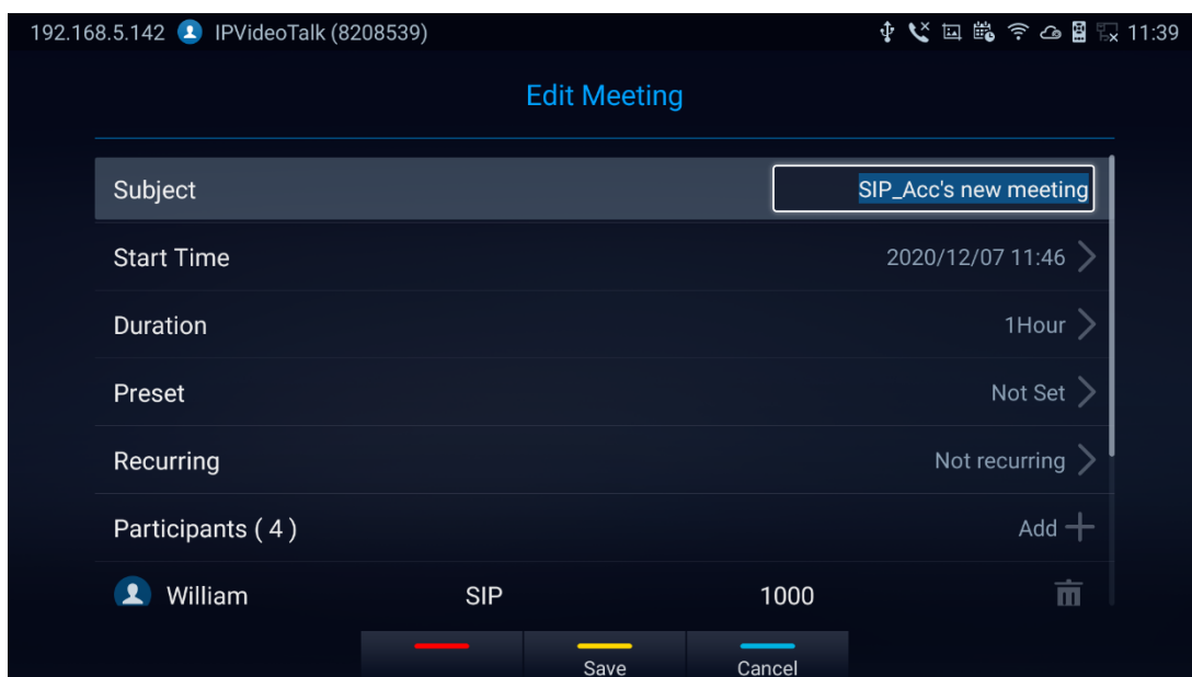
Figure 80: Edit conference
