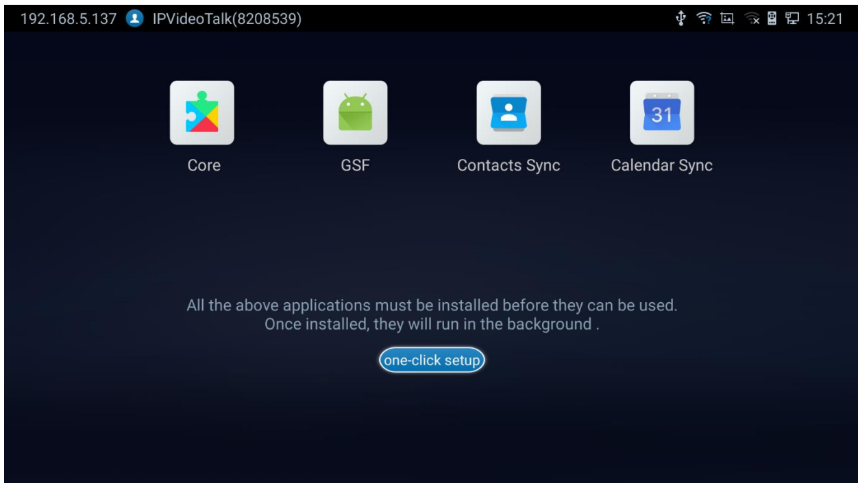
Figure 143: GMS Installation
