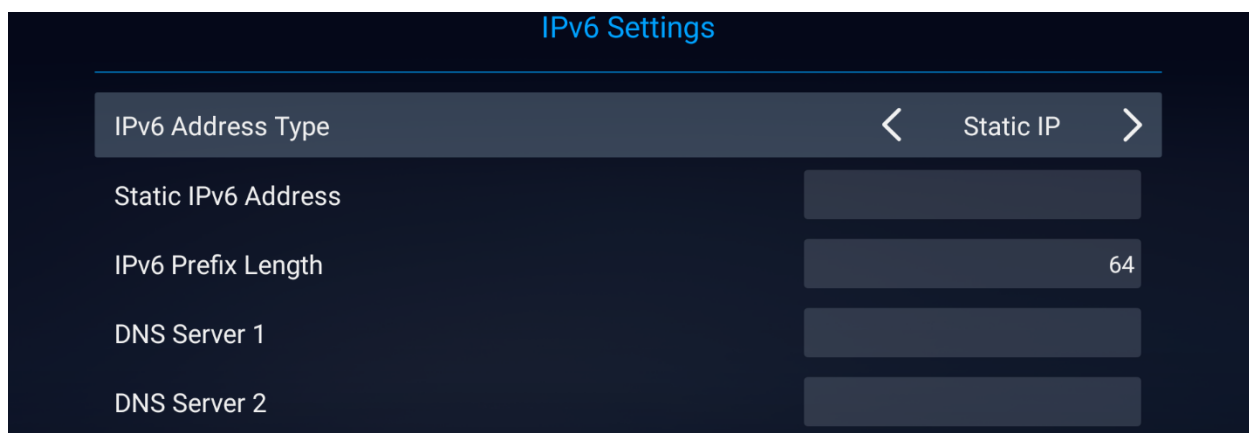
Figure 23: IPv6 Settings - Static
