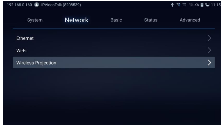
Figure 27: Wireless Projection
