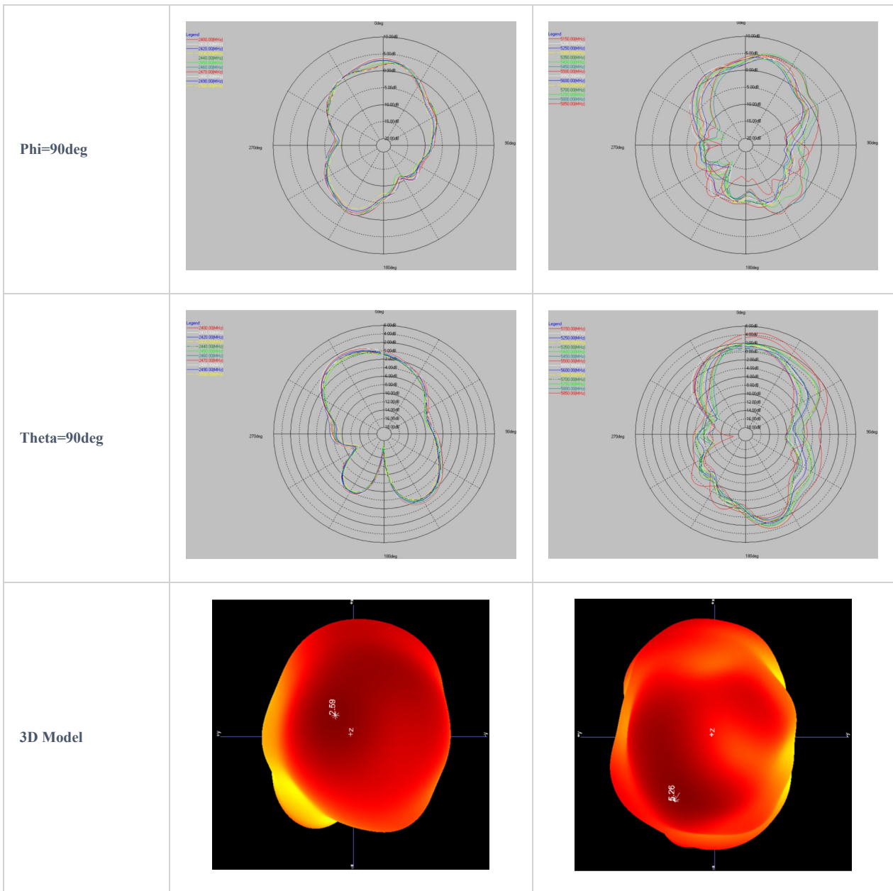
GWN7624 ANT1 Antenna Radiation Patterns
