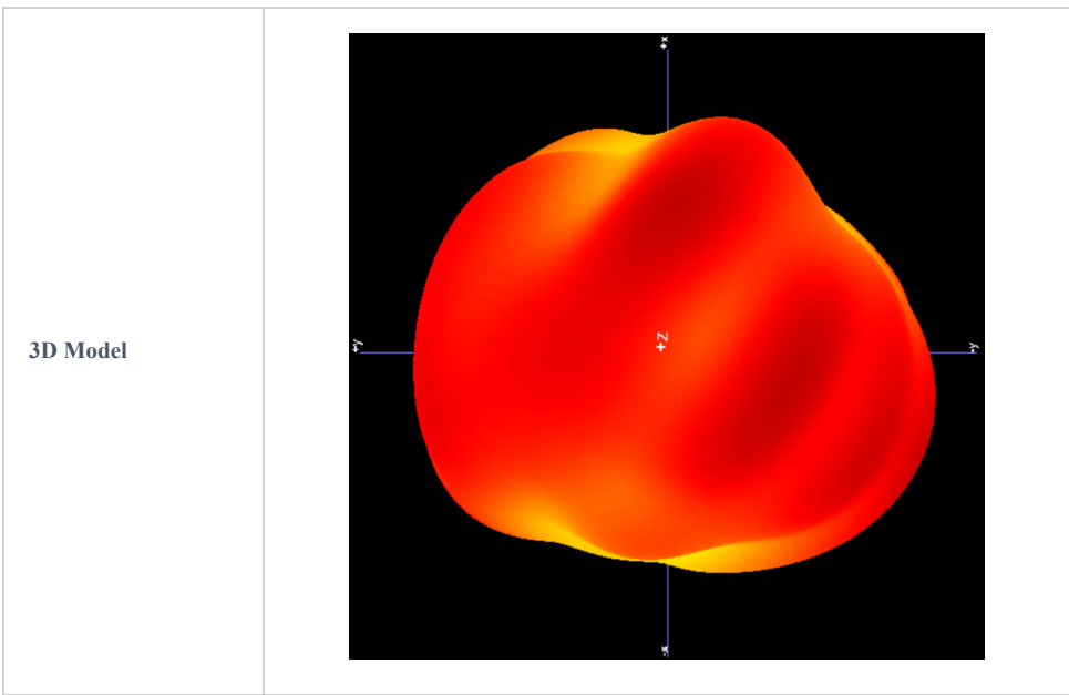
GWN7624 5G-1# Antenna Radiation Patterns
