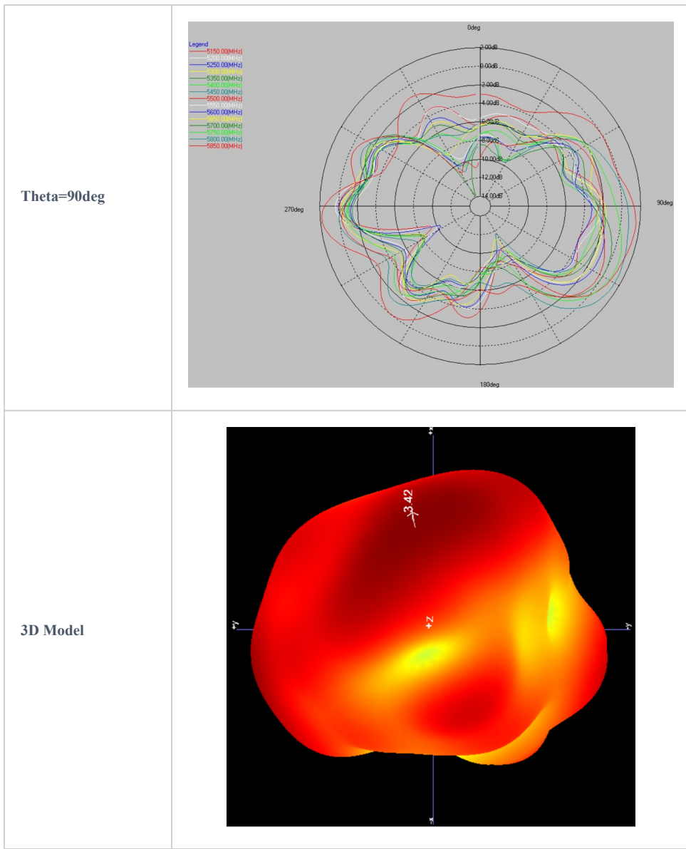
GWN7624 5G-2# Antenna Radiation Patterns
