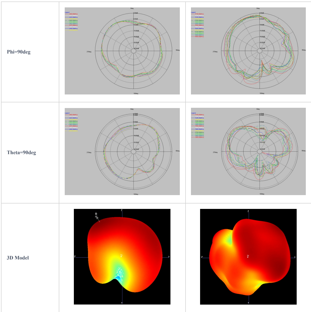
GWN7624 ANT2 Antenna Radiation Patterns
