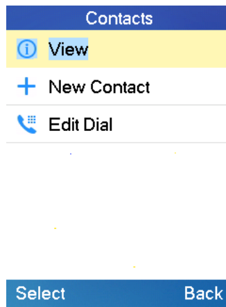
Figure 35: Contacts
