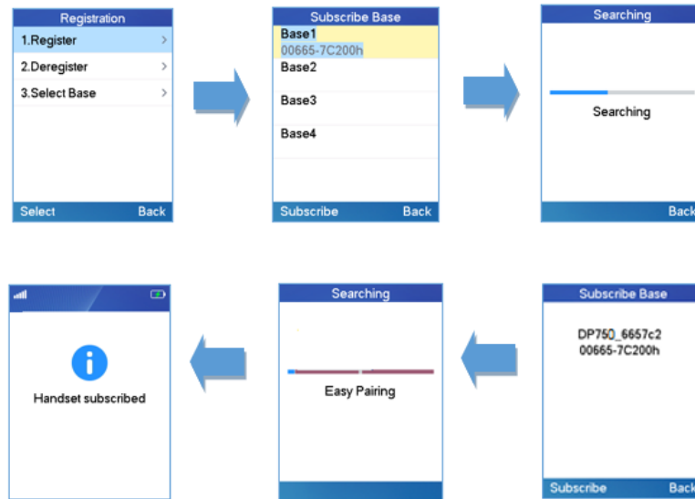
Figure 19: Registration Process
