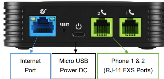
Figure 4: HT802 Back Panel
