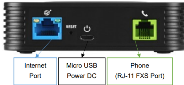
Figure 3: HT801 Back Panel
