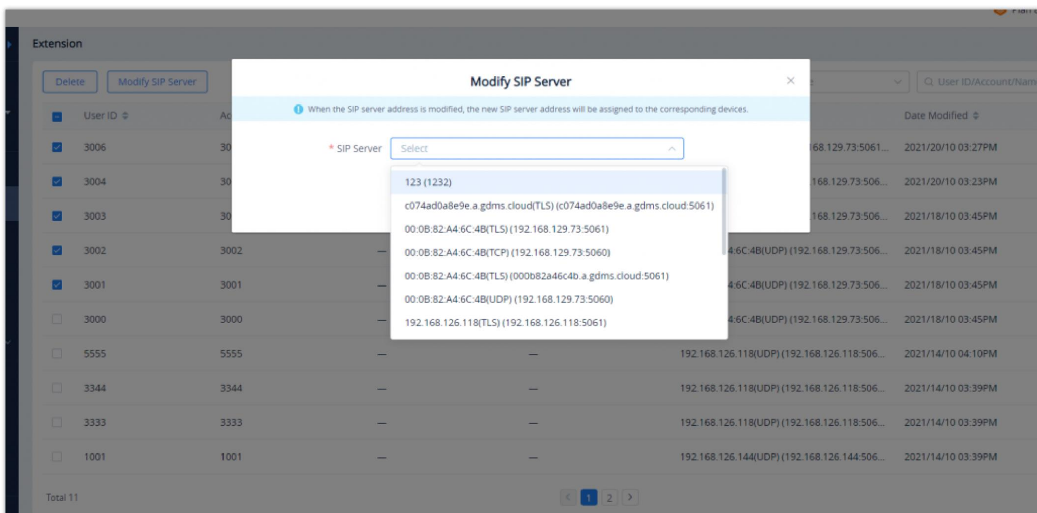
Modify SIP Server
