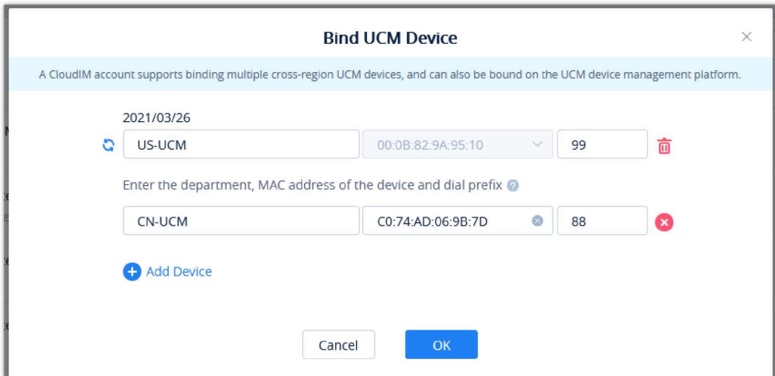
View Bound UCM Devices
