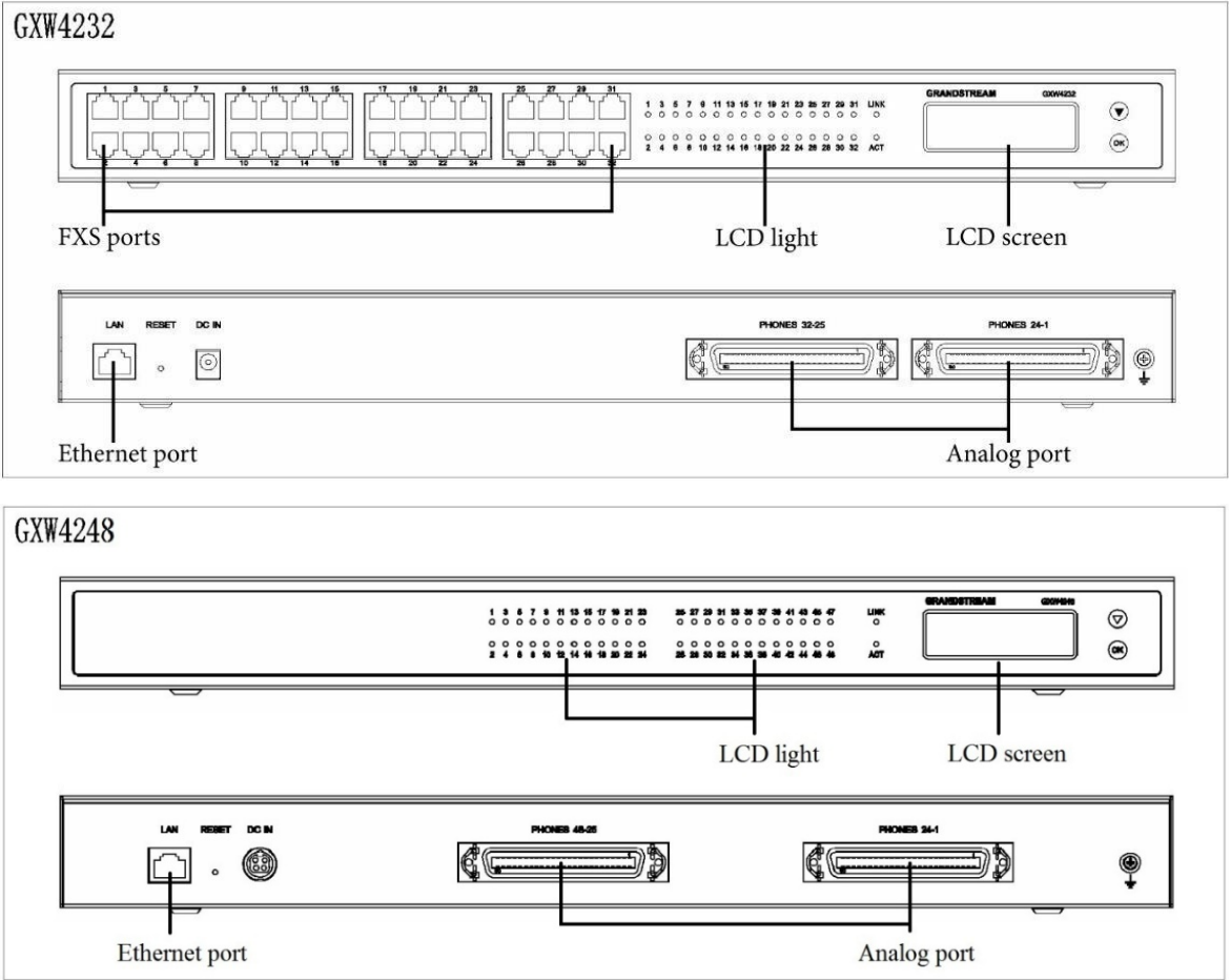
Figure 1: Diagram of GXW4216/24/32/48 Panel
