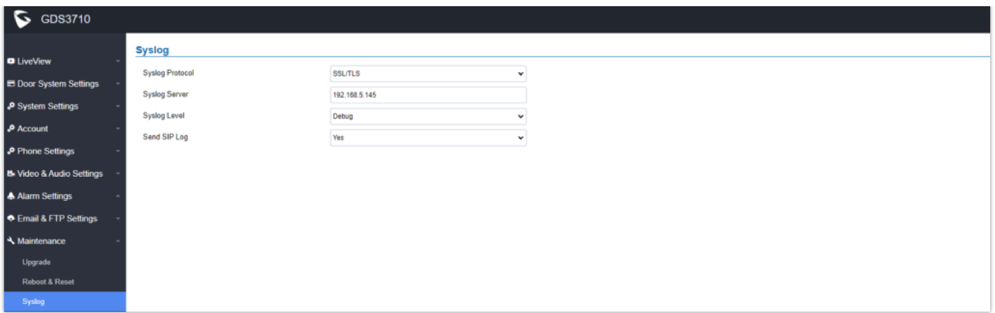
Syslog Page
