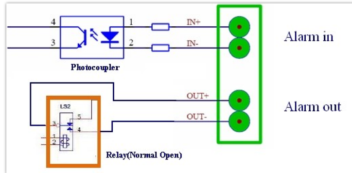
Alarm_In/Out Circuit for GDS371x
