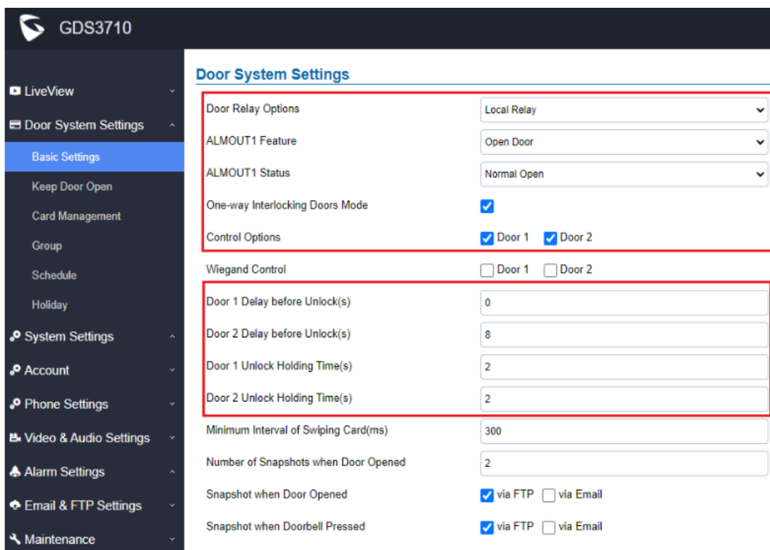
One-Way Interlocking Mode_GDS3710_Configuration_1
