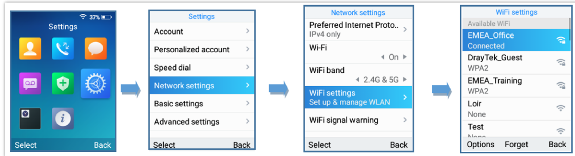
Figure 6: Wi-Fi Settings
