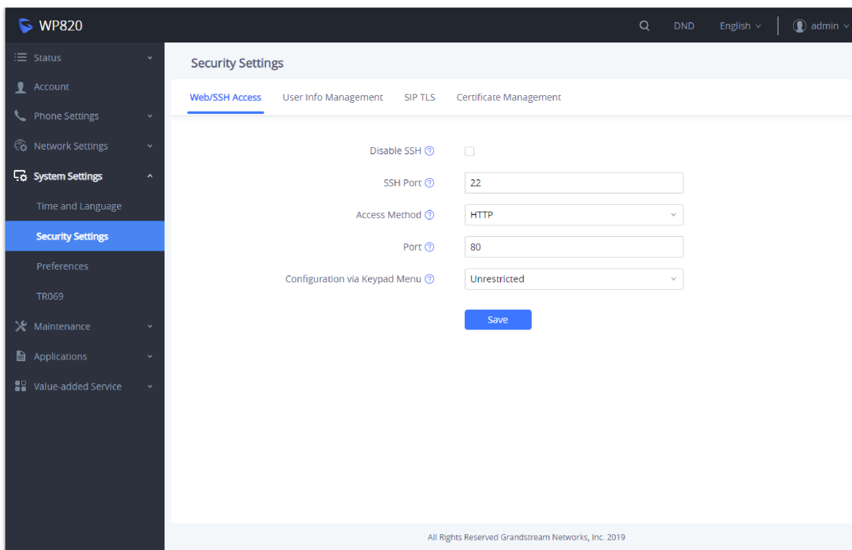
Figure 11: Web/SSH access
