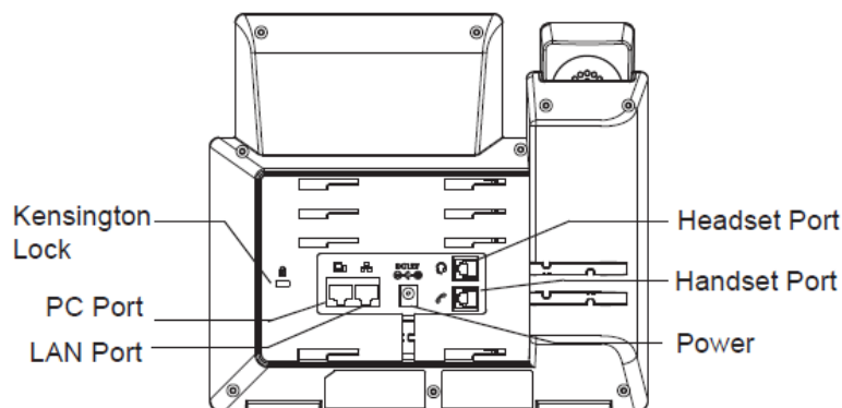
GRP261X/GRP2624/GRP263x/GRP2670/GRP2650 Back / Side View
