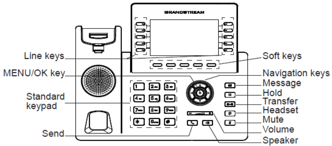
Figure 9: GRP2615 Keyboard
