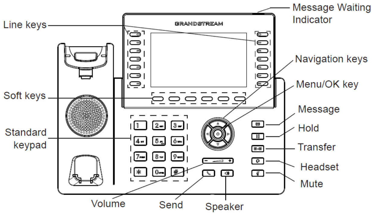
Figure 14: GPR2650 keypad
