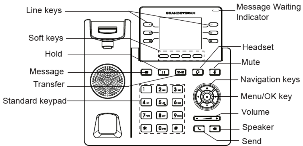
Figure 7: GRP2613 Keyboard
