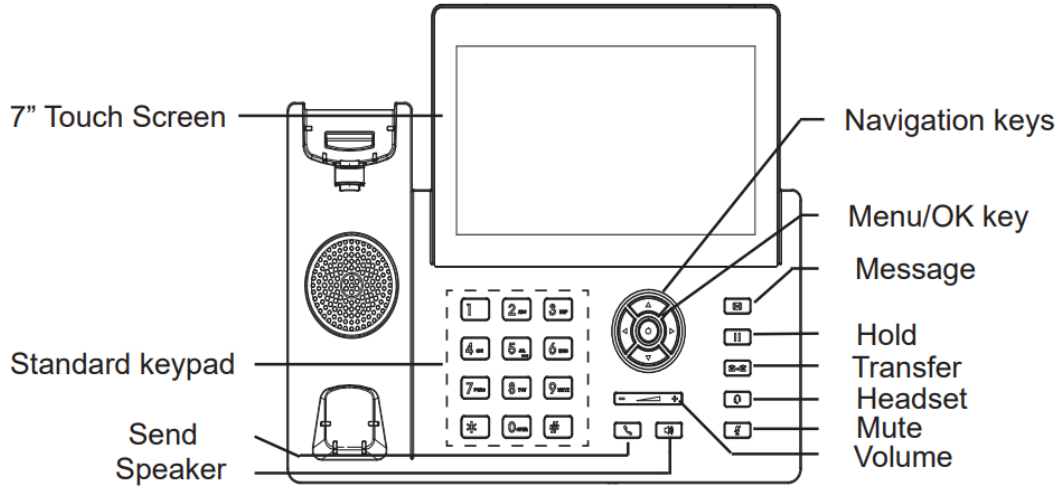
Figure 13: GRP2670 keypad
