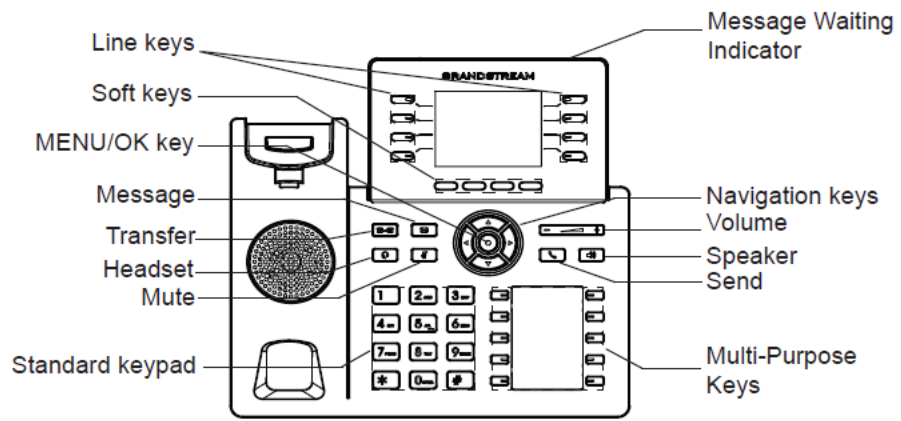
Figure 12: GRP2634 Keyboard
