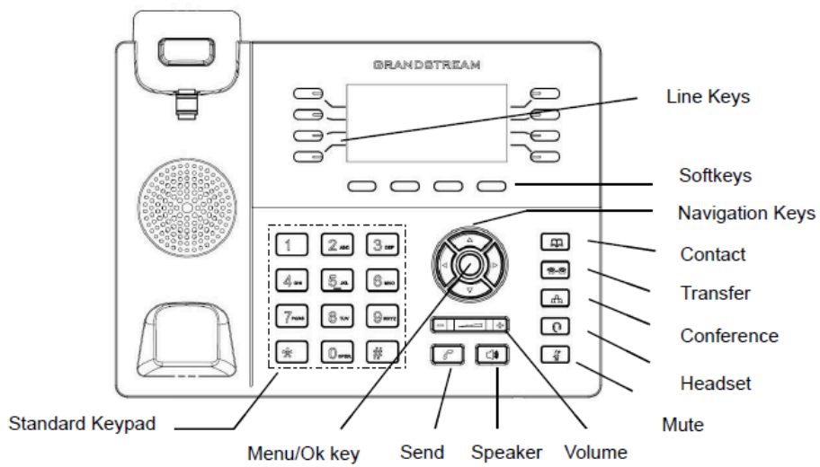
Figure 7: GXP1780/GXP1782 Keyboard
