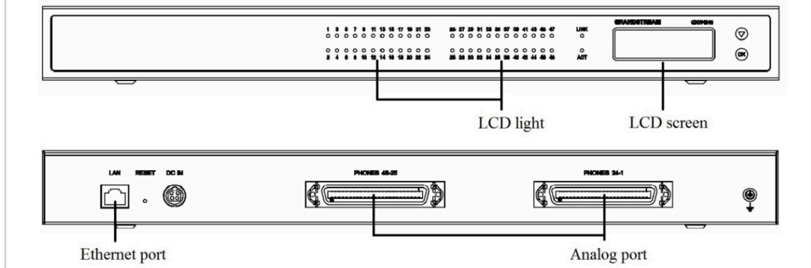
Diagram of GXW4216/24/32/48 Panel
