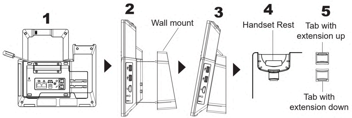
GXV3470 Wall Mount
