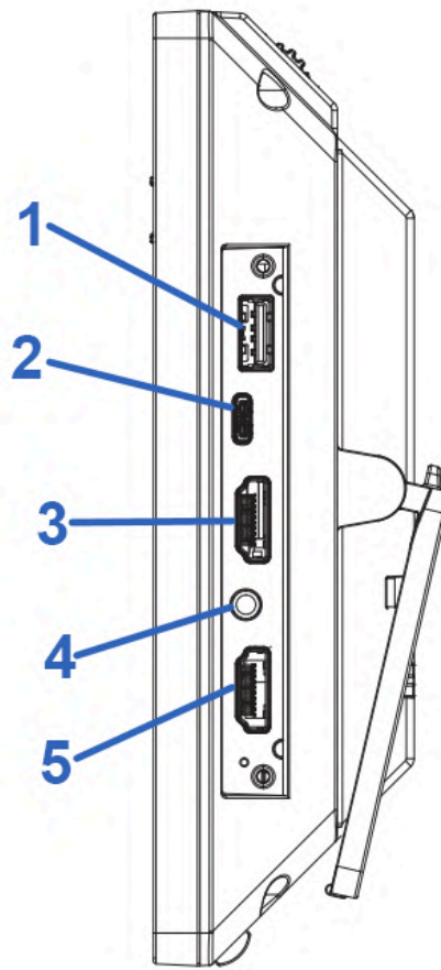
GXV3480 Side View
