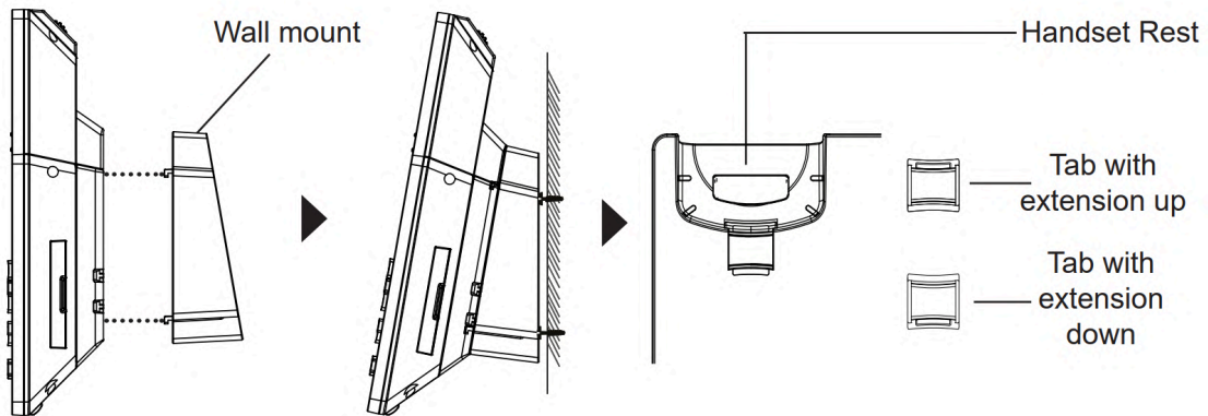
GXV3450 Wall Mount
