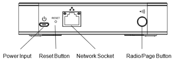
Figure 2: DP760 Back View
