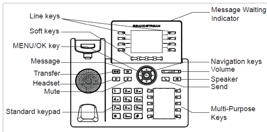
GRP2634 Keyboard
