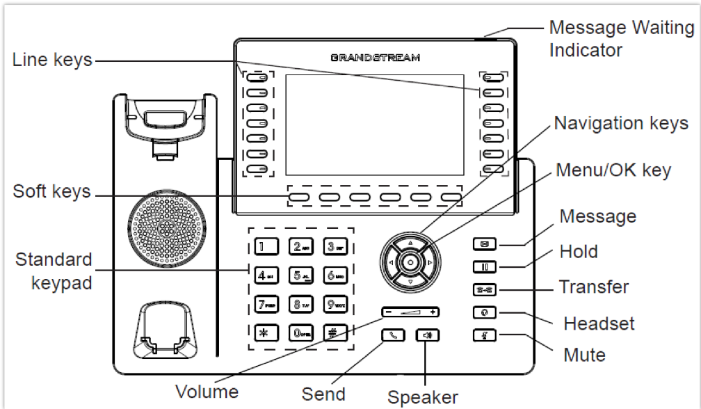
GRP2650 Keyboard
