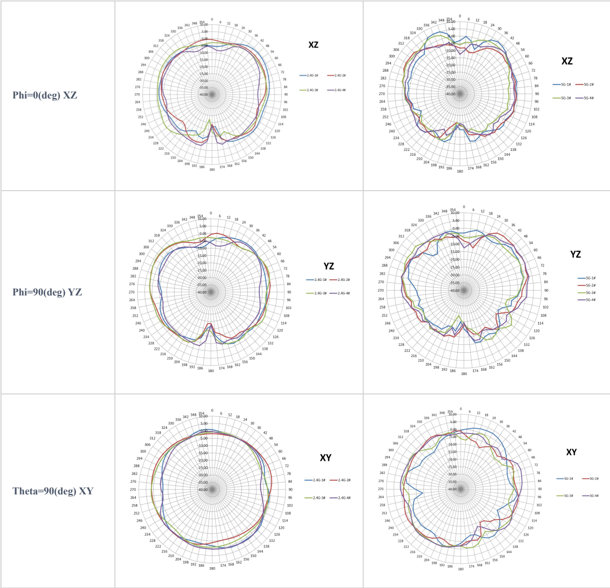
GWN7664 Antenna Radiation Patterns
