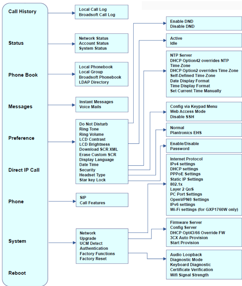
Keypad MENU Configuration
