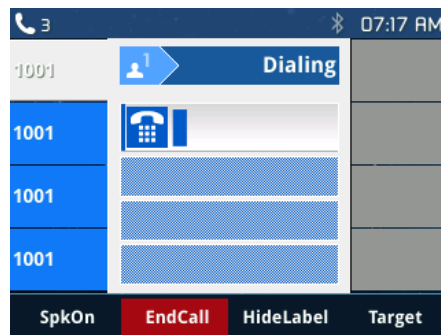
Figure 39: Group listening
