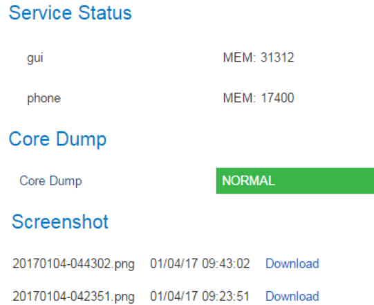
Figure 71: Screenshots
