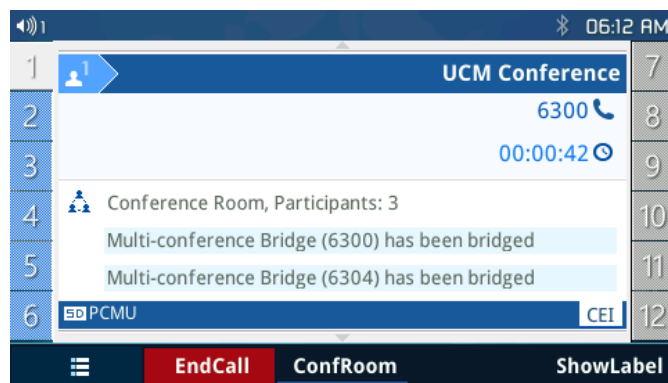
Figure 64: Conference Bridge
