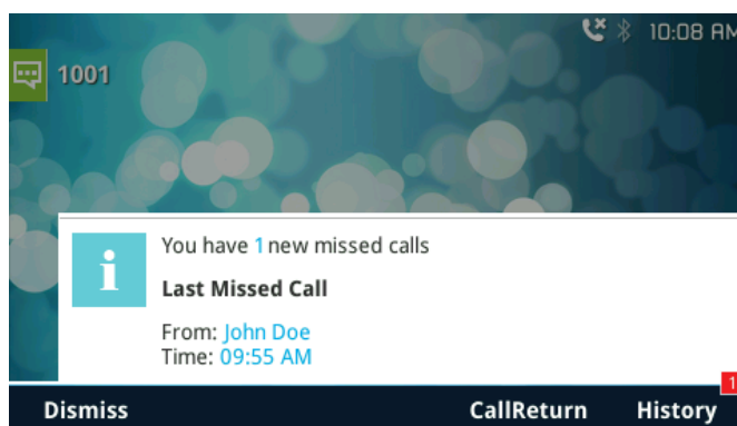
Figure 70: Missed Calls
