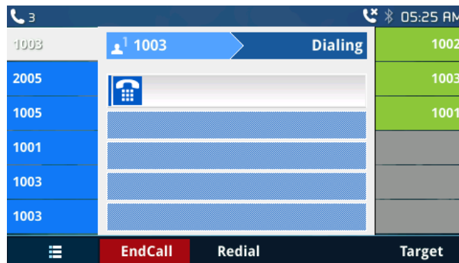
Figure 52: VPK Paging
