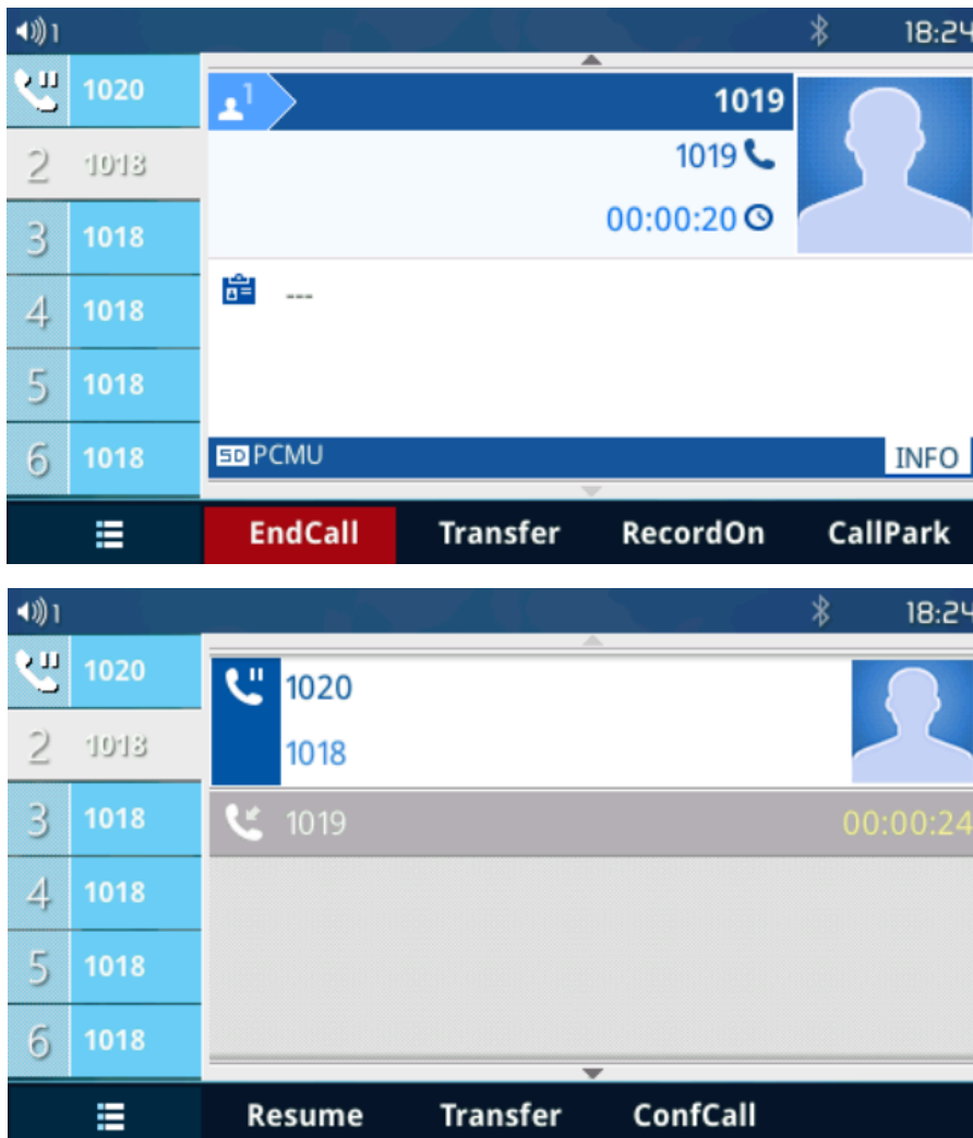
Figure 54: Line Switching
