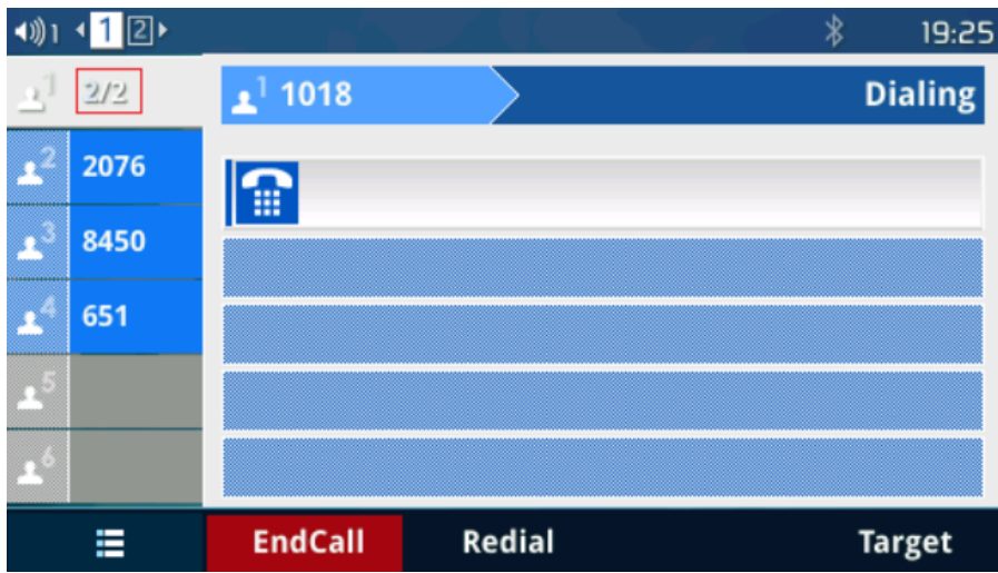
Figure 56: Account Mode
