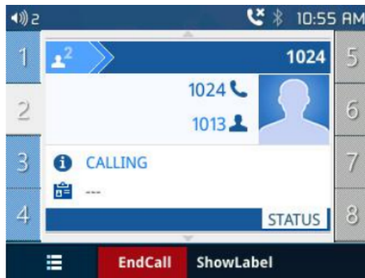
Figure 35: Show/Hidden Labels
