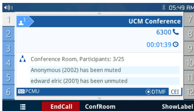
Figure 63: Mute/Unmute Conference
