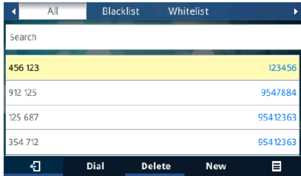
Figure 26: Before Search
