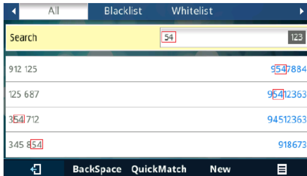
Figure 27: After Search
