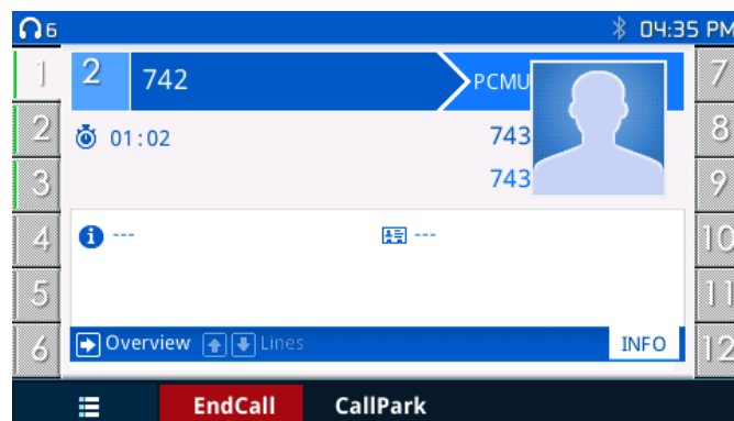
Figure 20: Making Call
