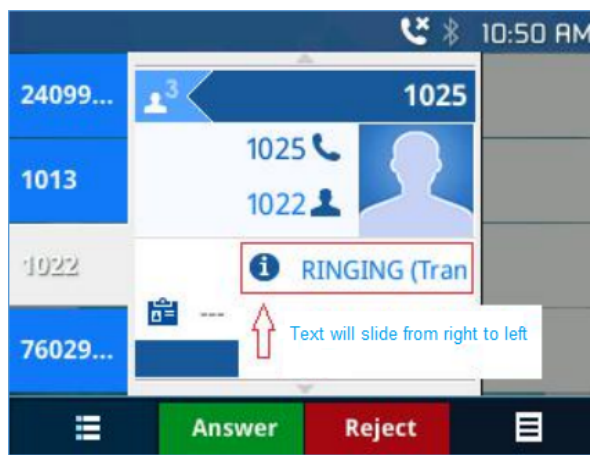
Figure 38: Text sliding
