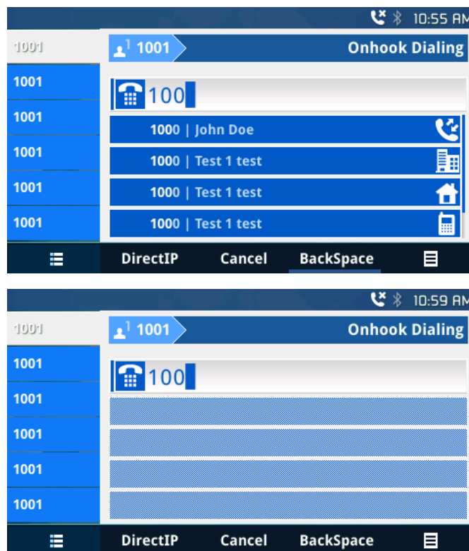
Figure 36: Predictive Dialing
