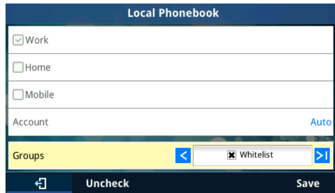
Figure 41: Black/White List
