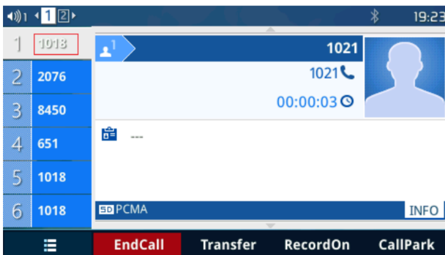
Figure 55: Line Mode
