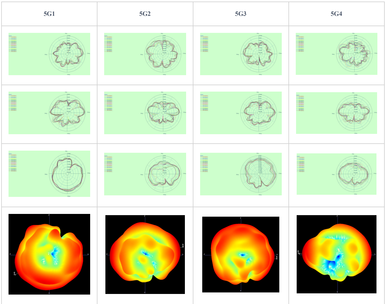
GWN7664ELR 5Ghz Antenna Radiation Patterns
