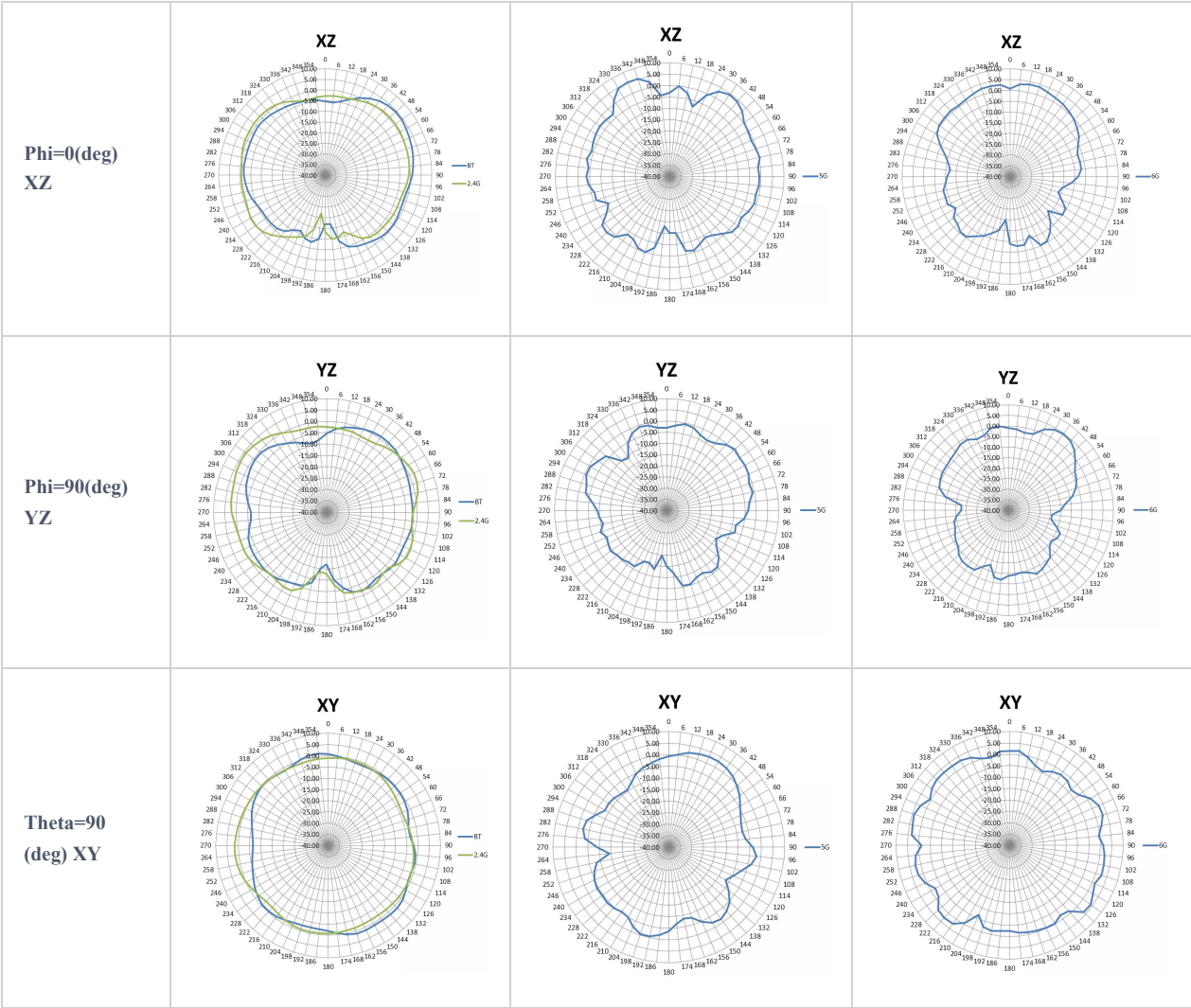
GWN7665 Antenna Radiation Patterns
