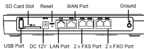
Figure 2: UCM6202 Back View
