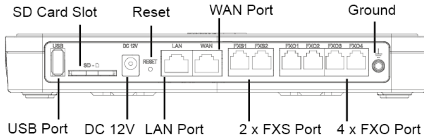
Figure 4: UCM6204 Back View
