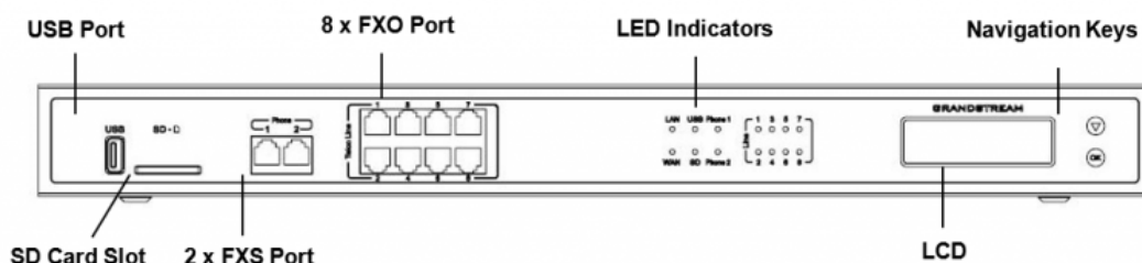
Figure 5: UCM6208 Front View
