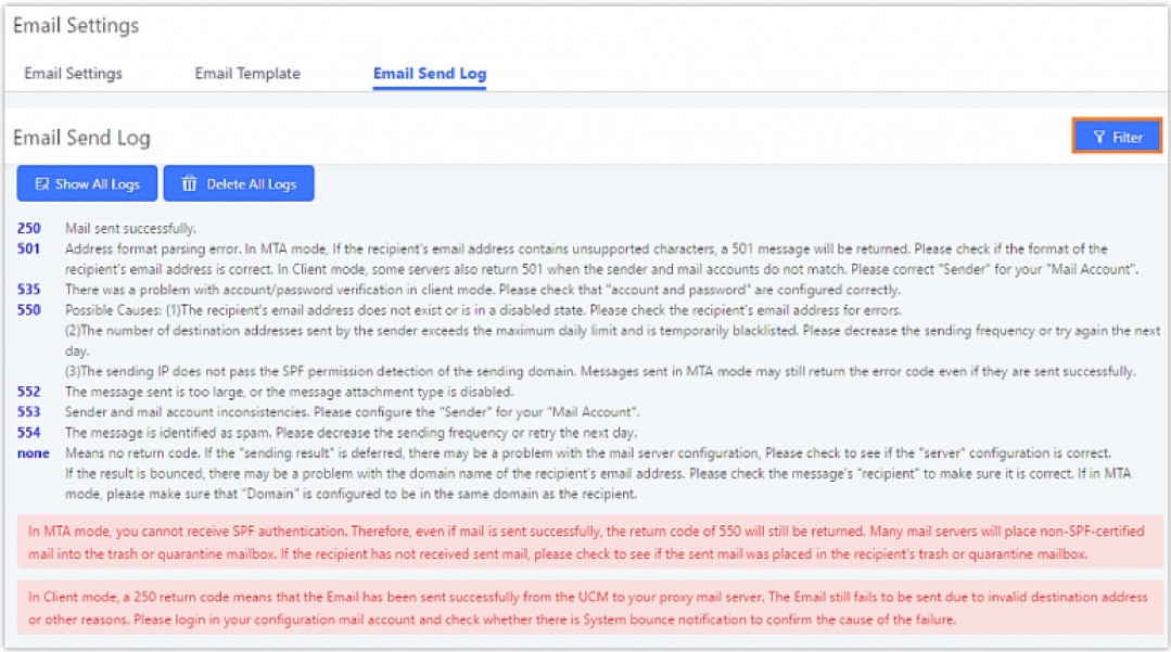
Figure 52: Email Send log
