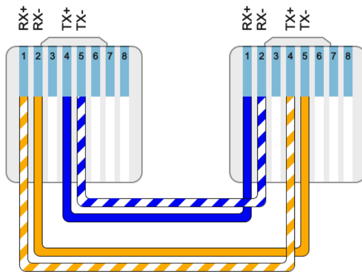
Figure 3: UCM6510 T1/E1/J1 Crossover Cable Pin-out
