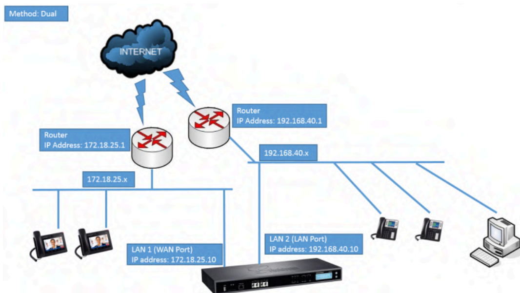
Figure 11: UCM6510 Network Interface Method: Dual
