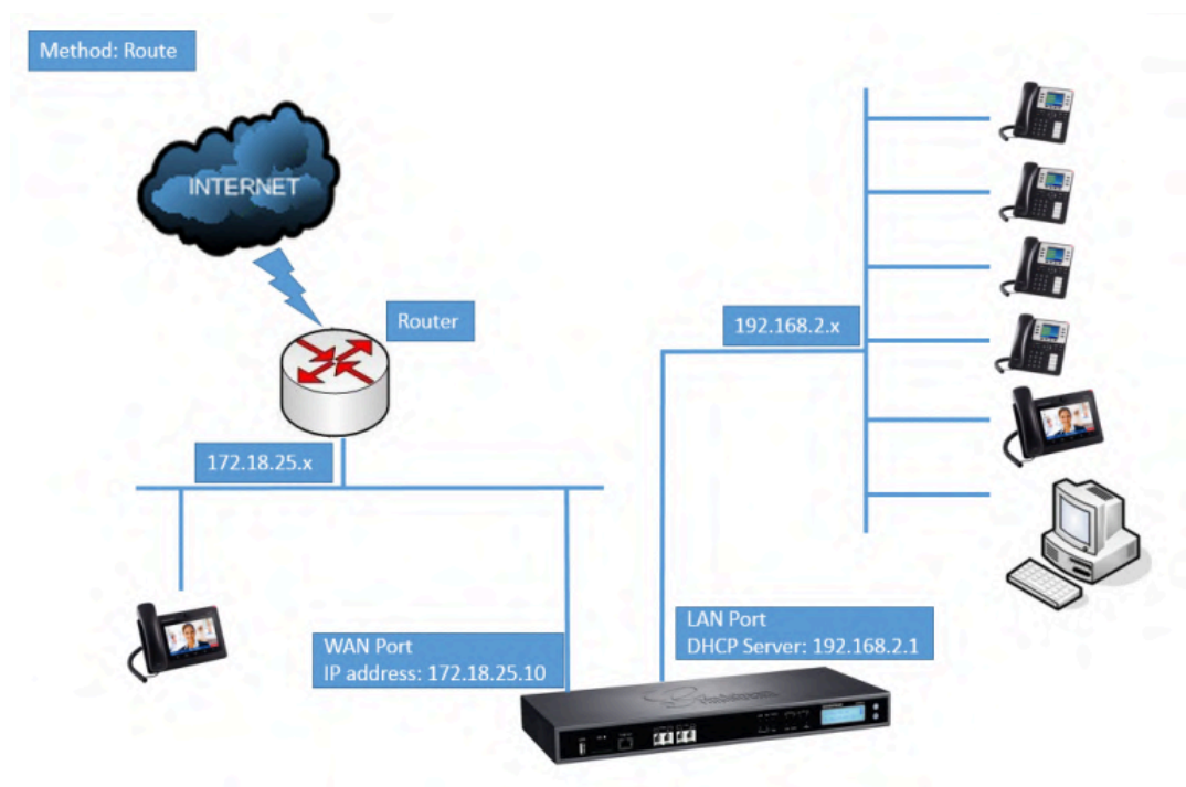
Figure 9: UCM6510 Network Interface Method: Route
