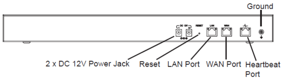
Figure 2: UCM6510 Back View
