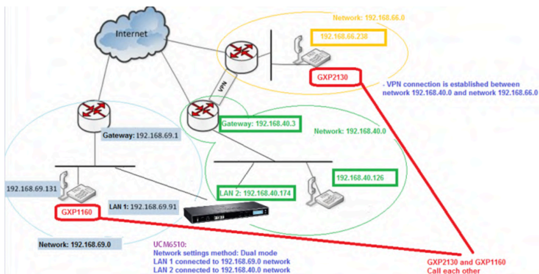
Figure 17: UCM6510 Static Route Sample
