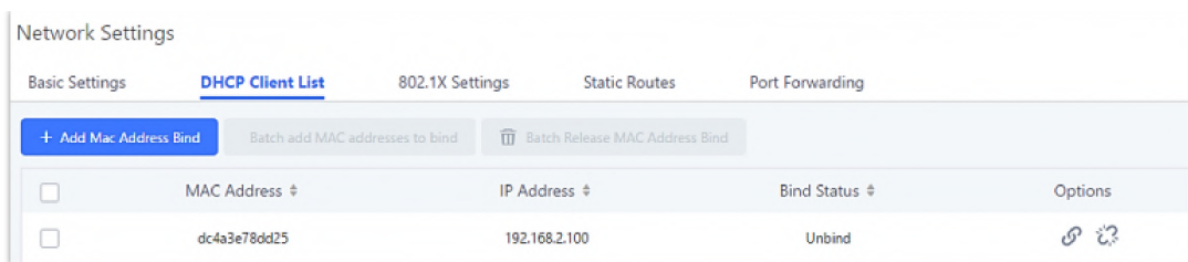
Figure 12: DHCP Client List
