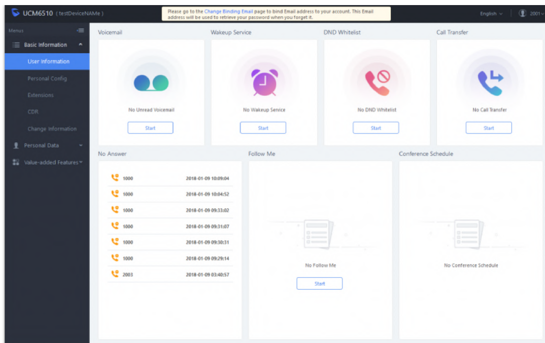
Figure 313: User Portal Layout
