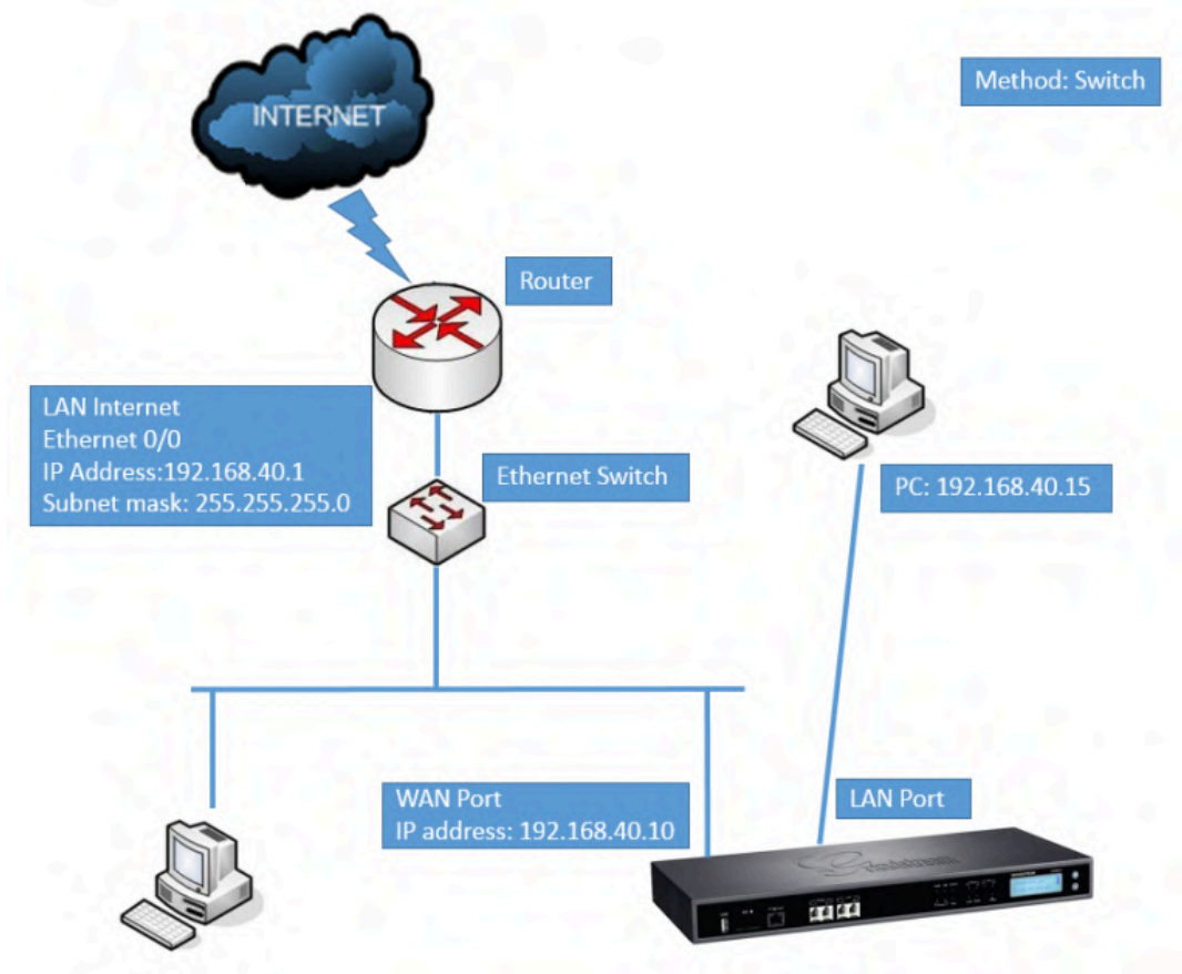
Figure 10: UCM6510 Network Interface Method: Switch
