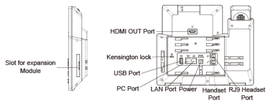
Figure 6: GXV3350 Back / Side View
