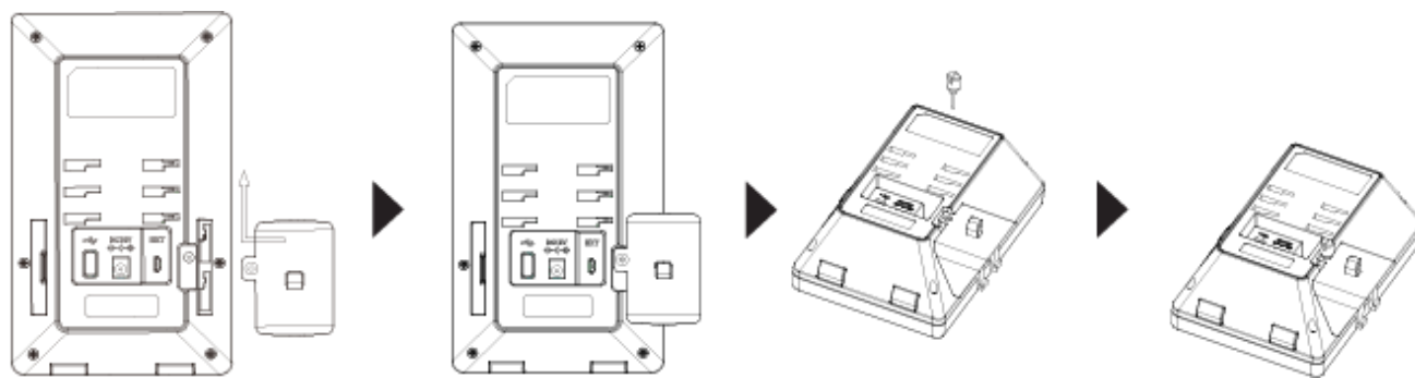
Figure 7: GBX20 with connector
