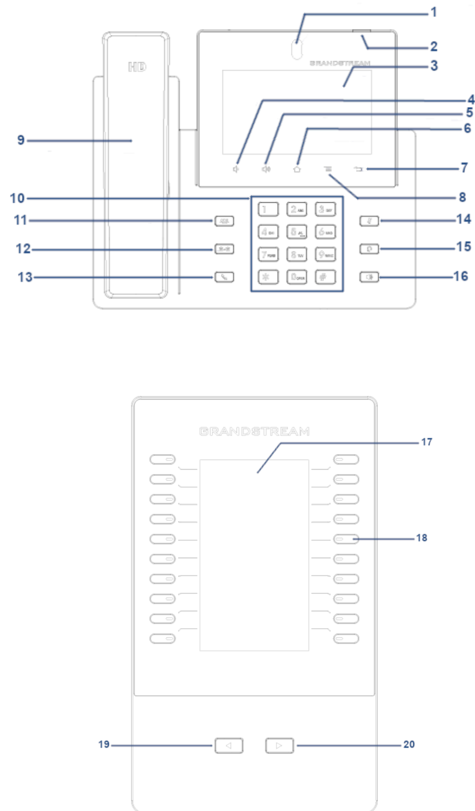
Figure 2: GXV3350 Front and GBX20 Extension Module Front
