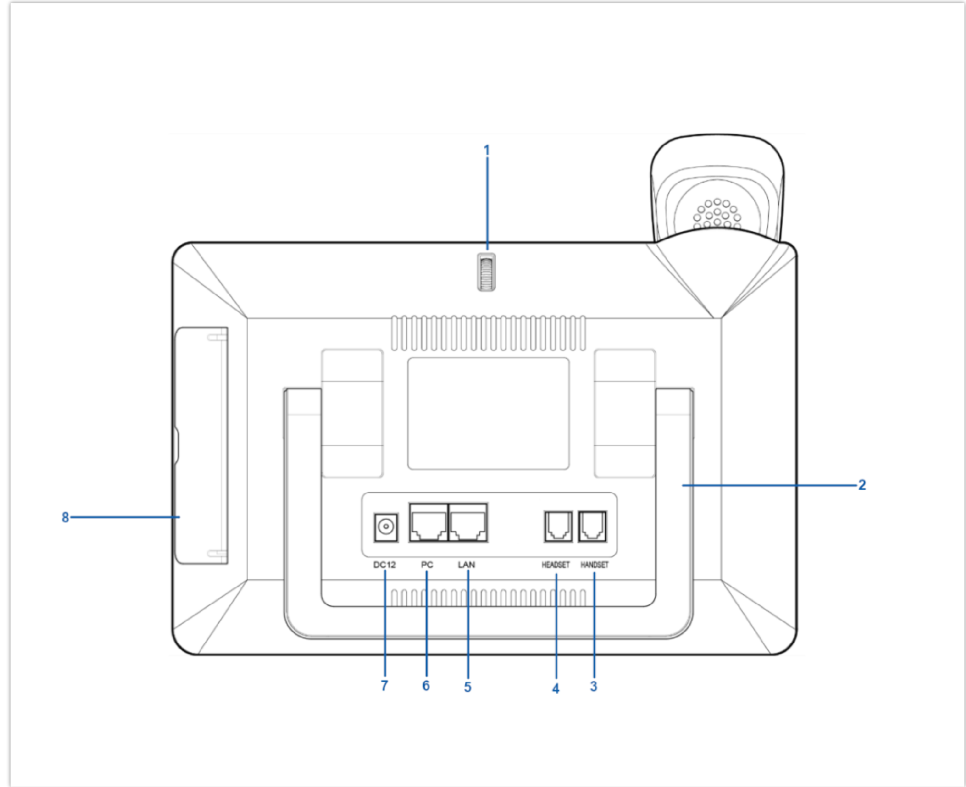
GXV3370 Back View
