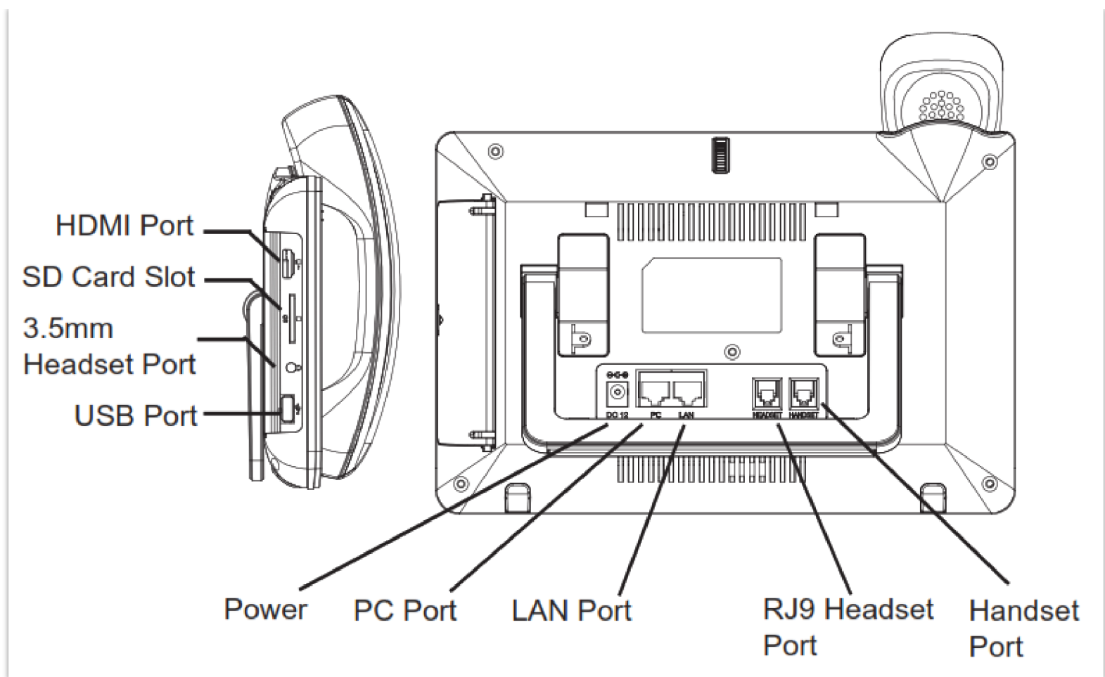
GXV3370 Back / Side View
