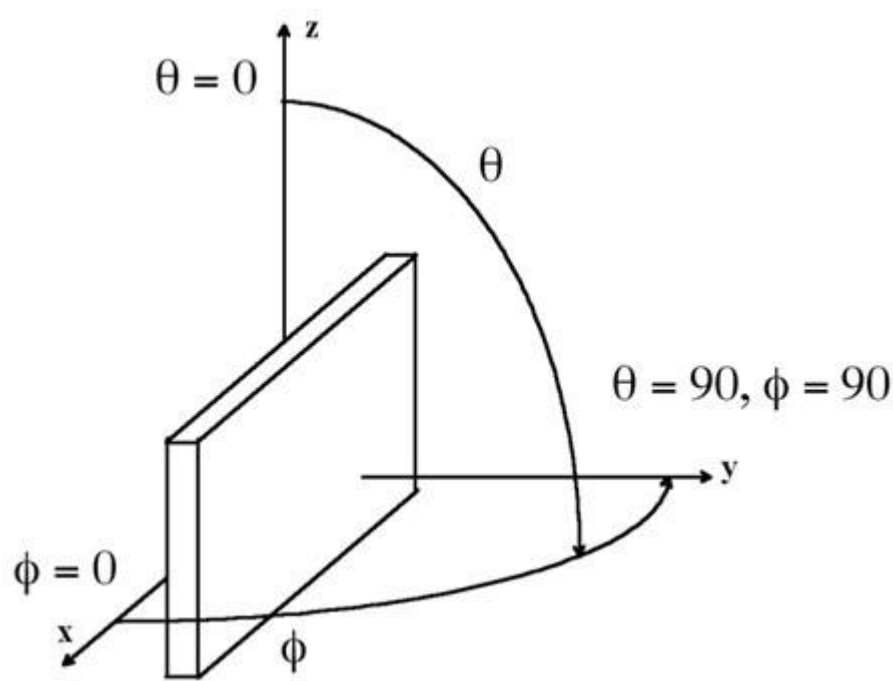
Figure 1: Polar Coordinates
