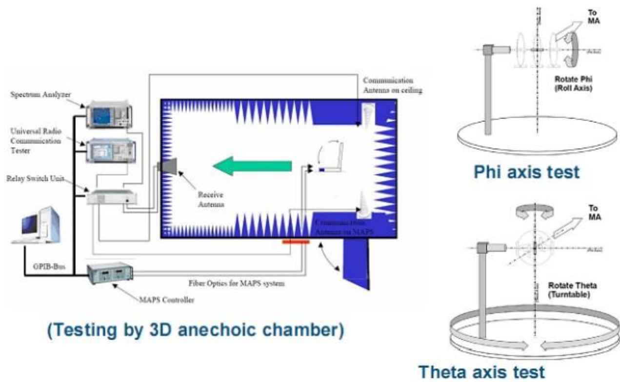
Figure 2 Test Environment
