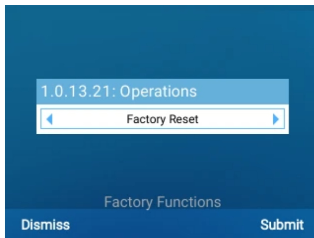
Factory Reset
