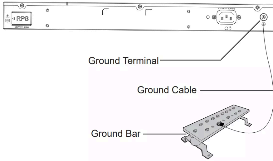
Grounding the Switch
