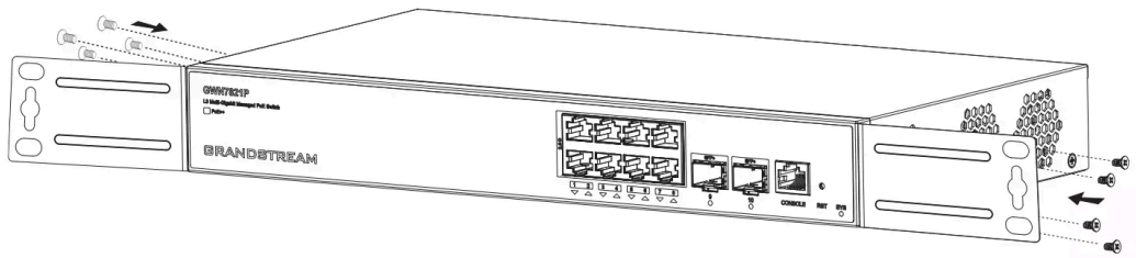
Install on 19 Standard Rack
