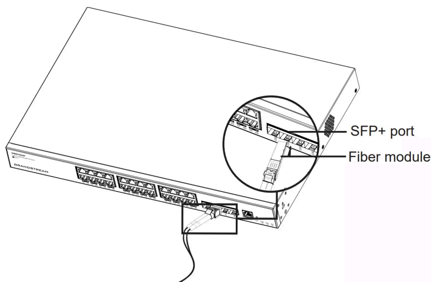
Connect to SFP+ port
