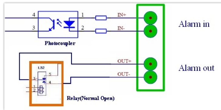
Alarm InOut Circuit
