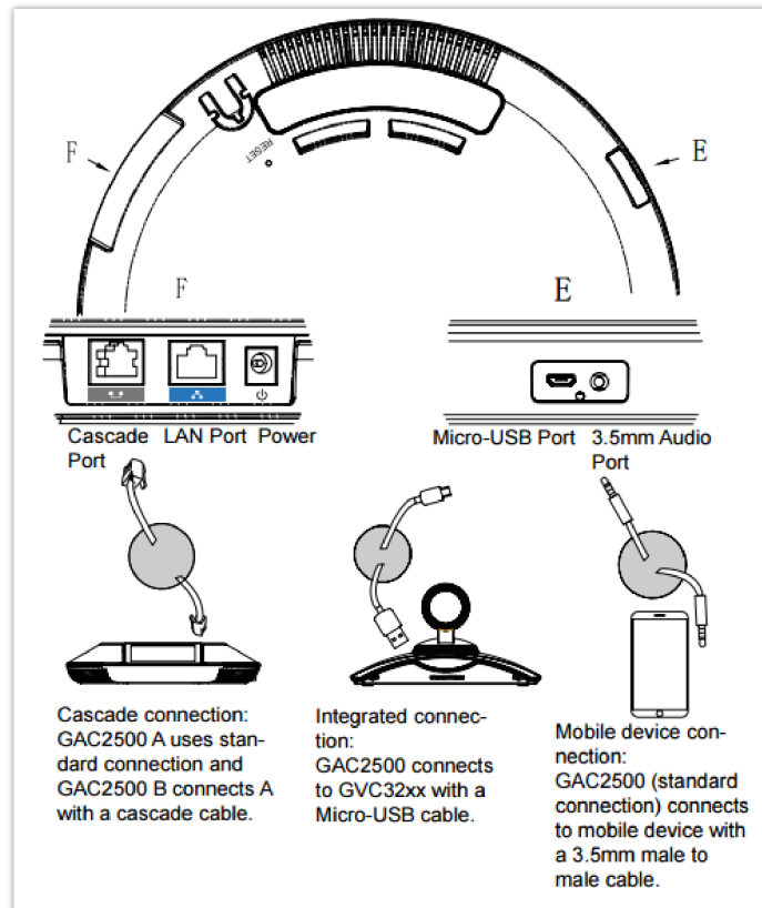
Connecting the GAC2500
