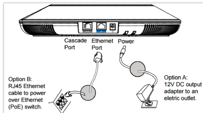
Powering the GAC2500
