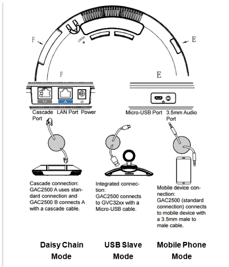
Connecting the GAC2500
