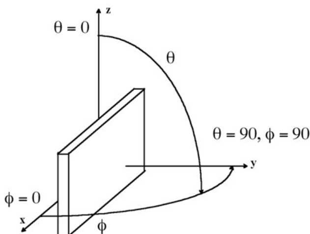
Figure 1: Polar Coordinates
