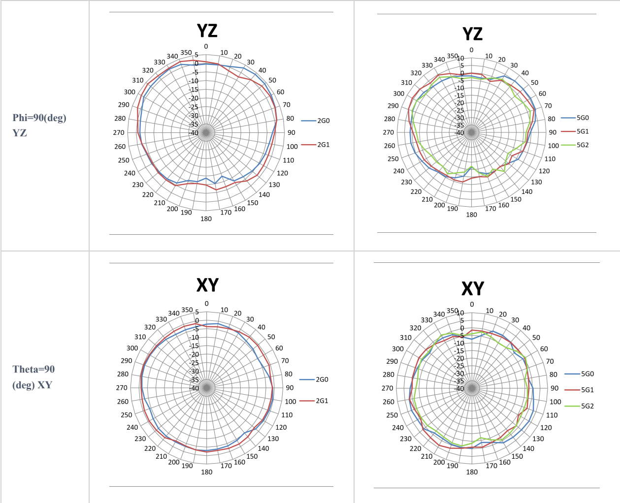
GWN7670E Antenna Radiation Patterns
