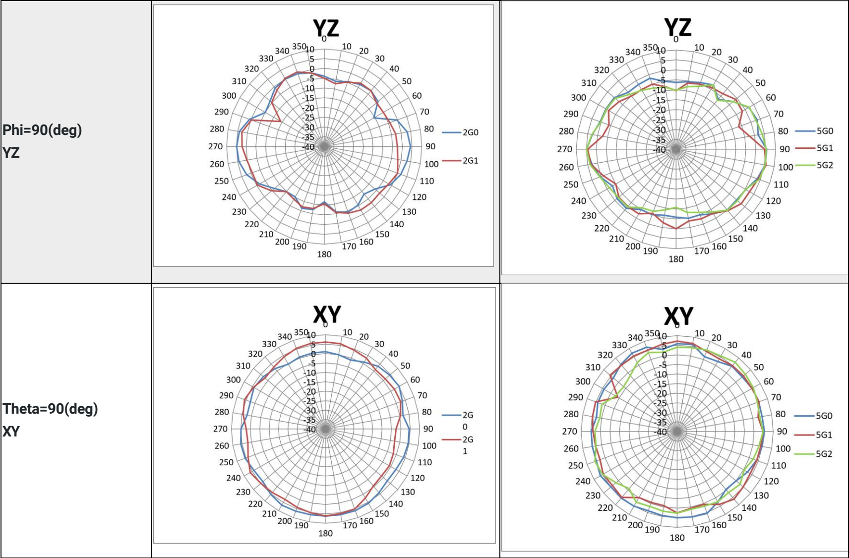
GWN7670ELR Antenna Radiation Patterns
