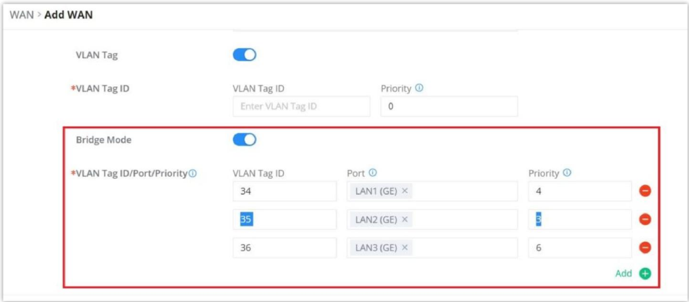
Bridge Mode
