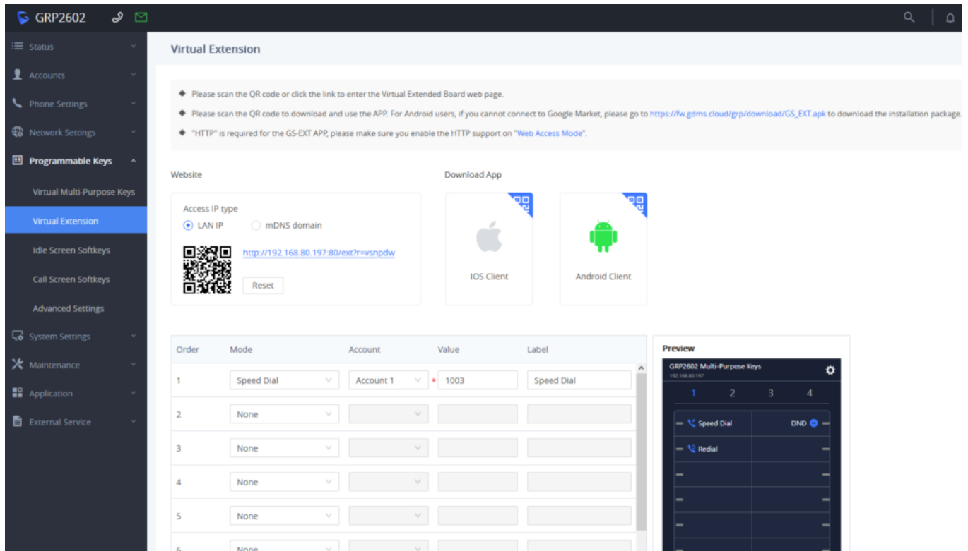
Virtual extensions Tab
