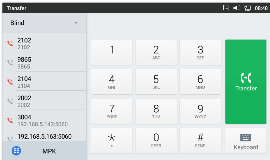
Figure 79 Attended Transfer
