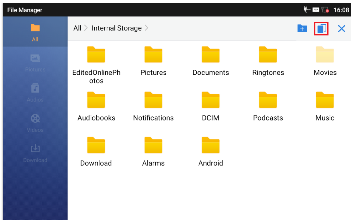
Figure 151 Paste File
