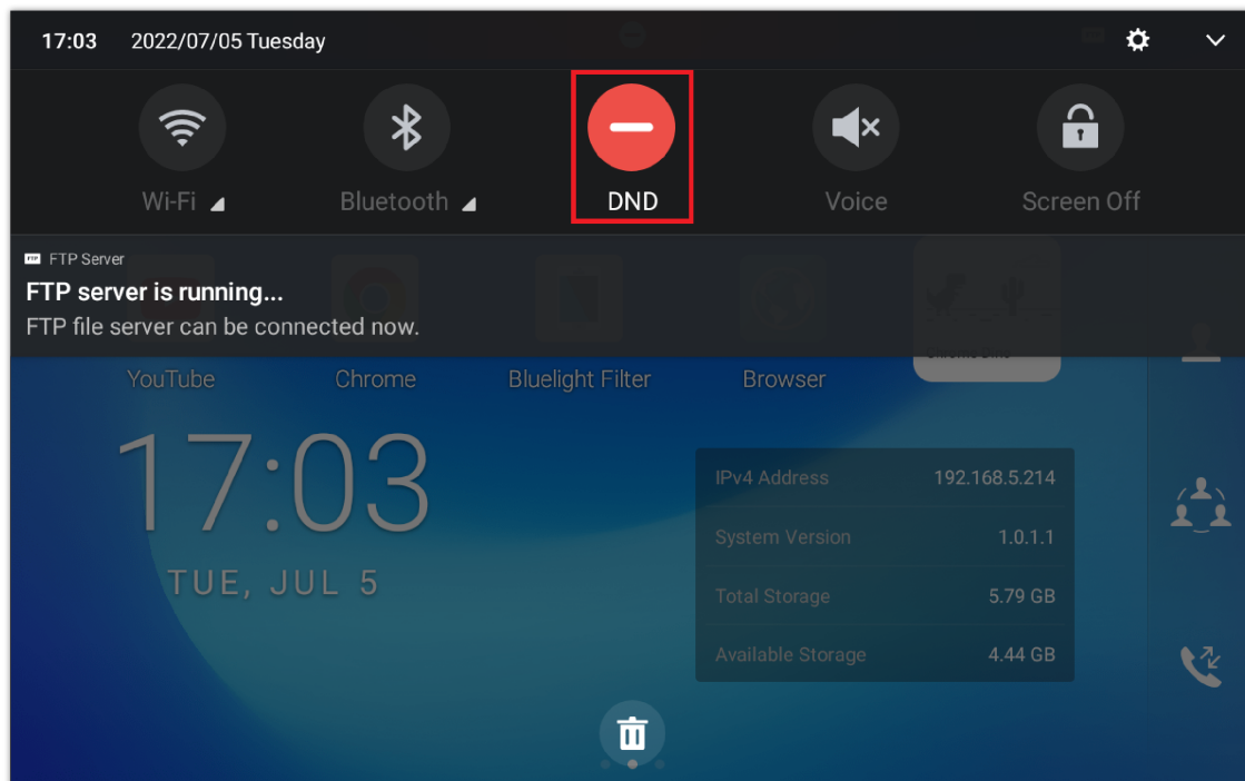
Figure 101 Enable/Disable DND
