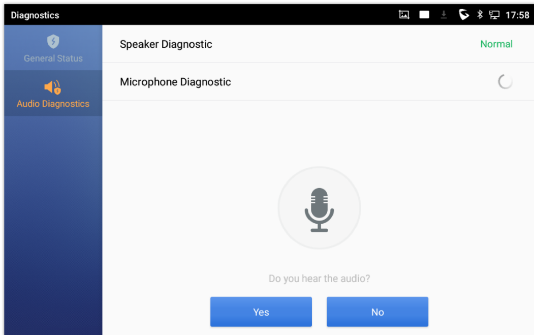
Microphone diagnosis
