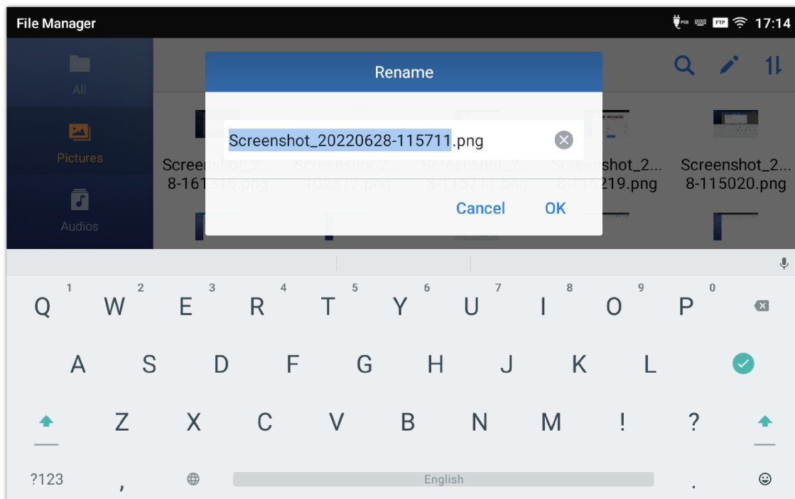
Figure 155 Rename File
