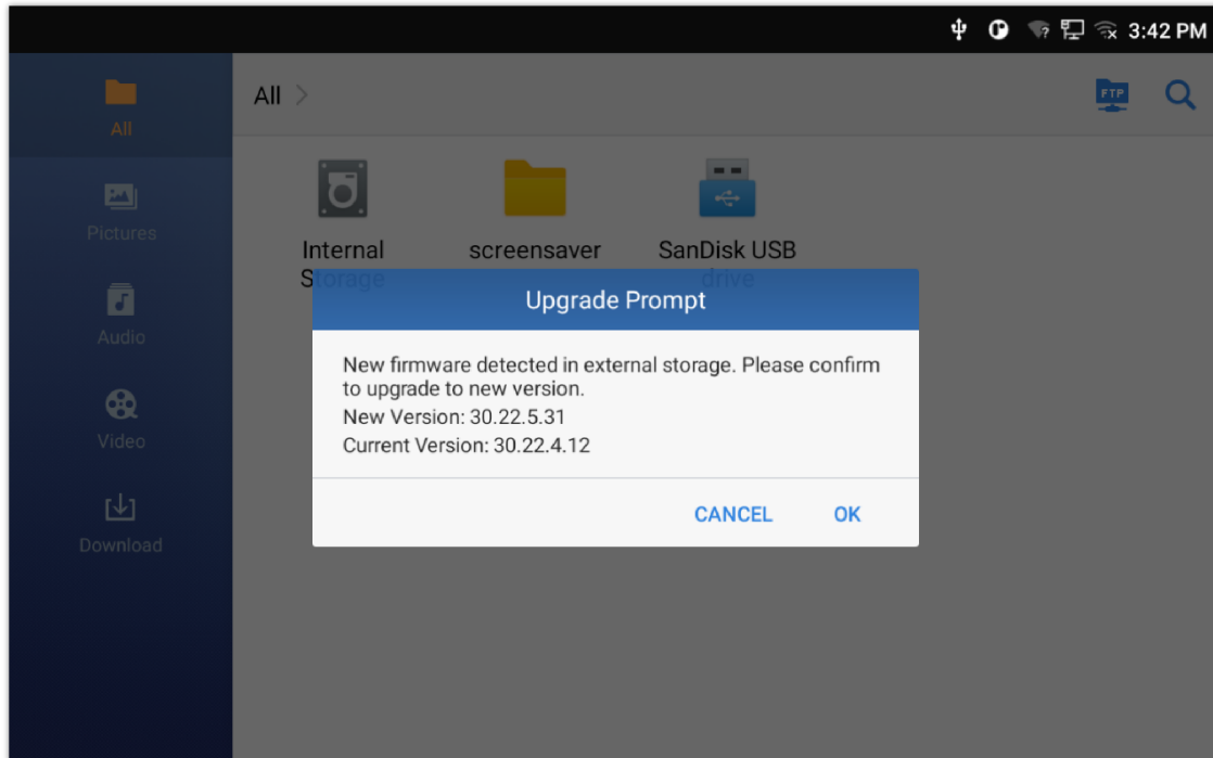
Figure 46 Upgrade Prompt
