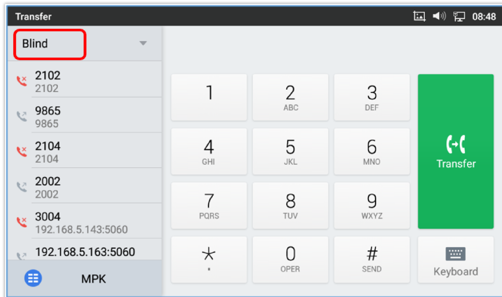
Figure 75 Blind Transfer
