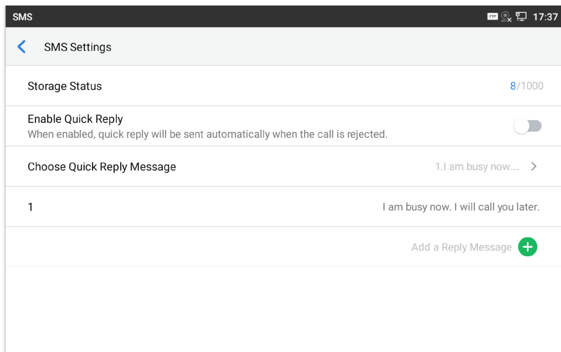
Figure 138 SMS Settings
