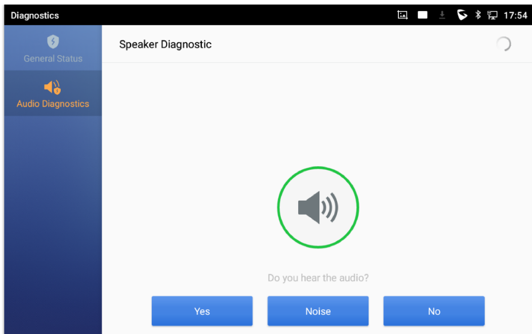
Figure 120 Speaker Diagnosis
