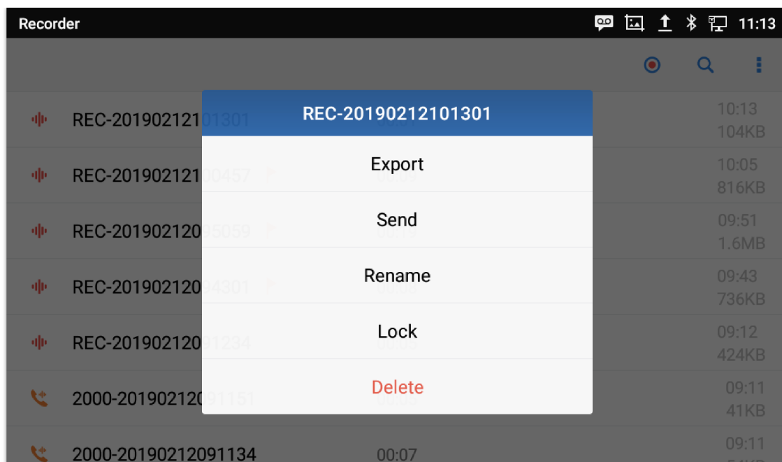
Figure 148 Files operation
