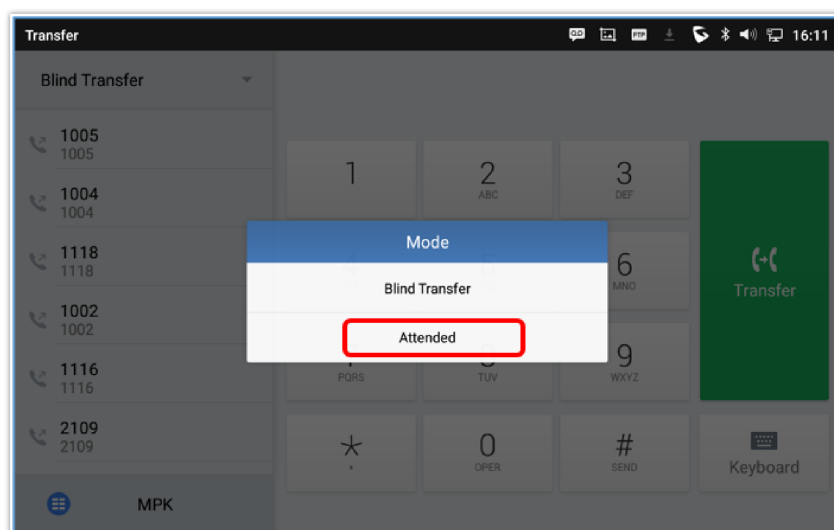
Figure 76 Attended Transfer
