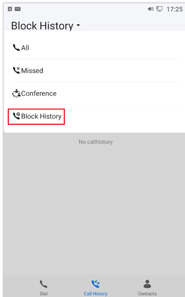
Figure 125 Block History
