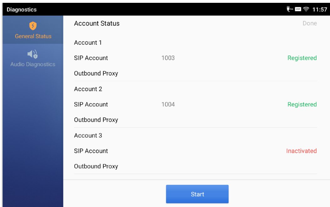
Figure 118 Account Status
