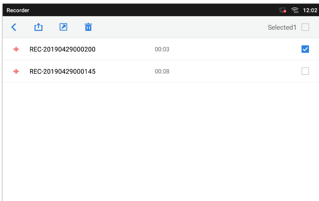
Figure 149 ExportDelete files
