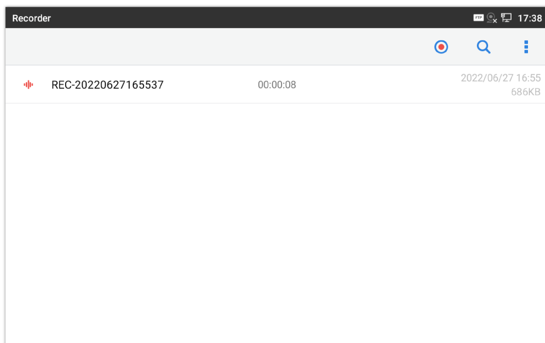
Figure 139 Recorder Application
