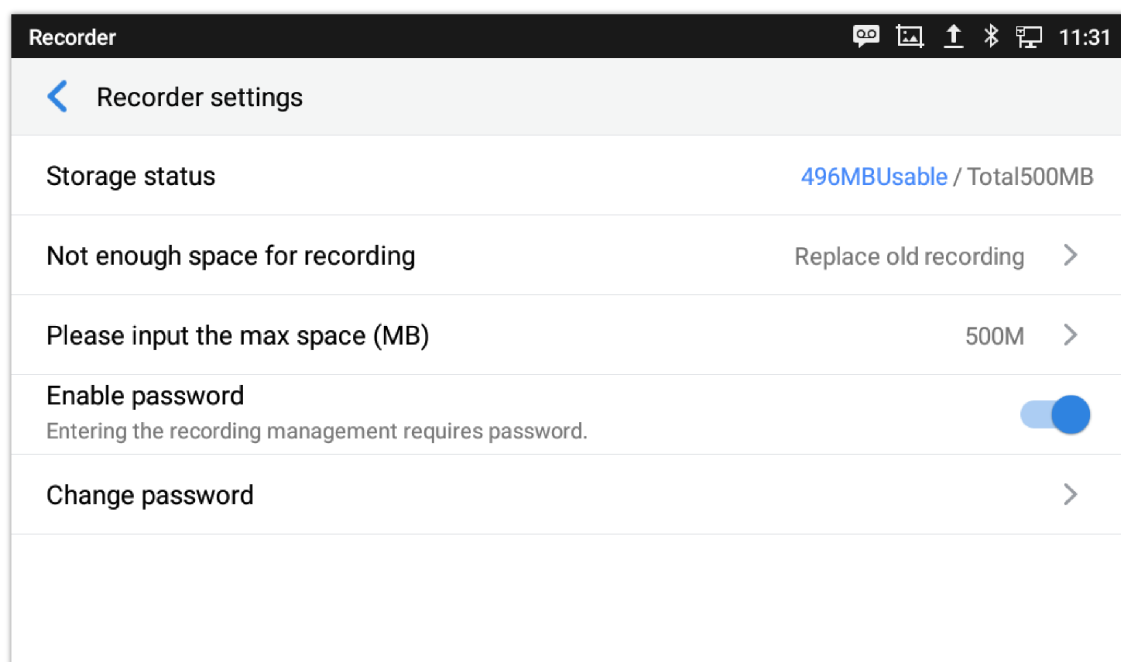
Figure 145 Recorder Settings
