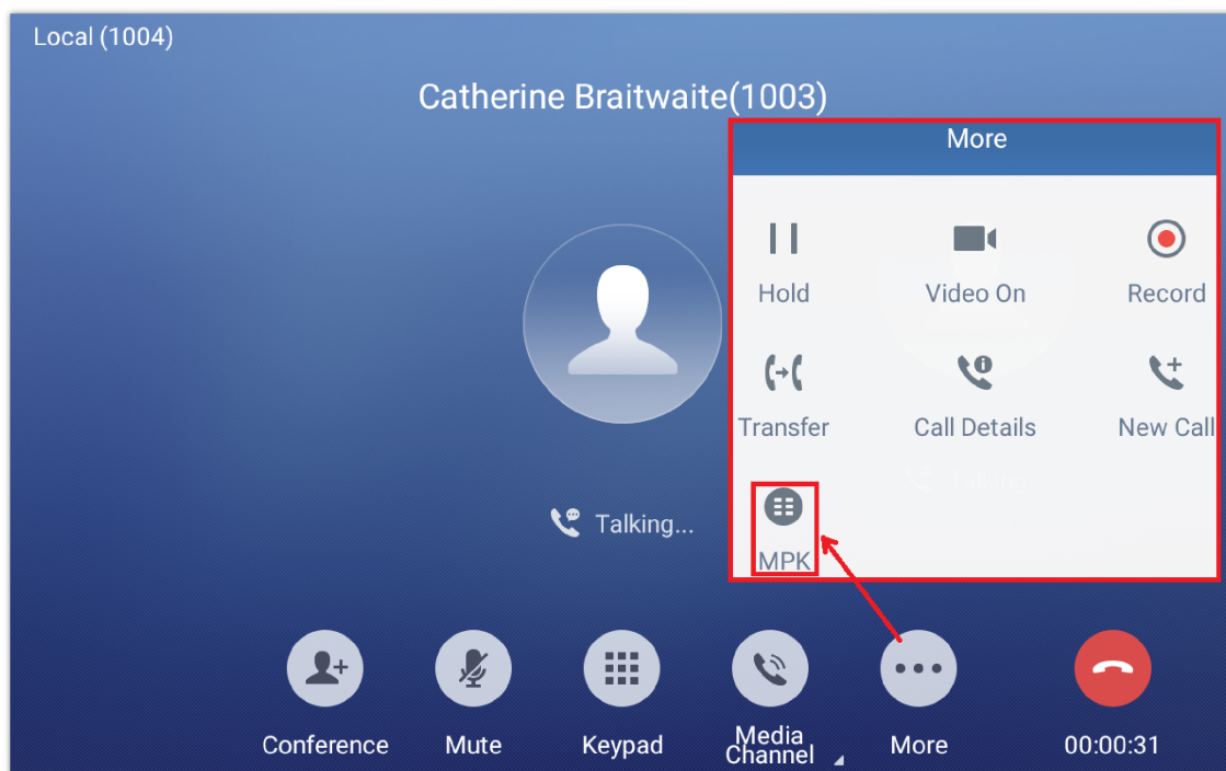
Figure 69 MPK button
