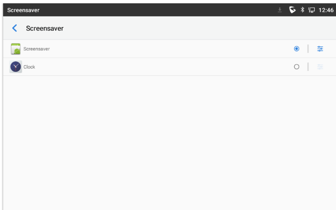
Figure 160 Screensaver settings
