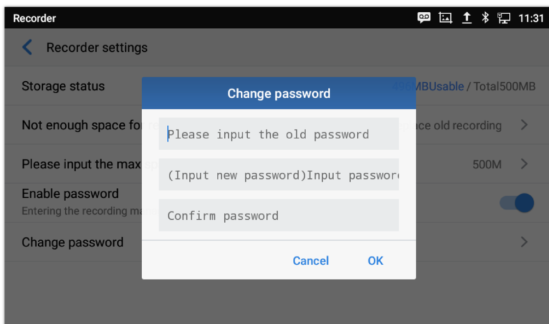
Figure 147 Change Password
