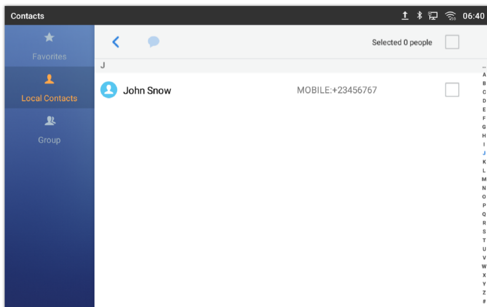
Figure 135 Select contact
