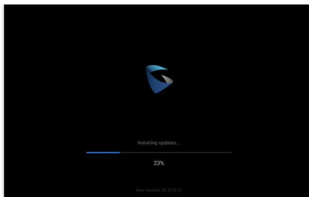
Figure 48 Installing Firmware
