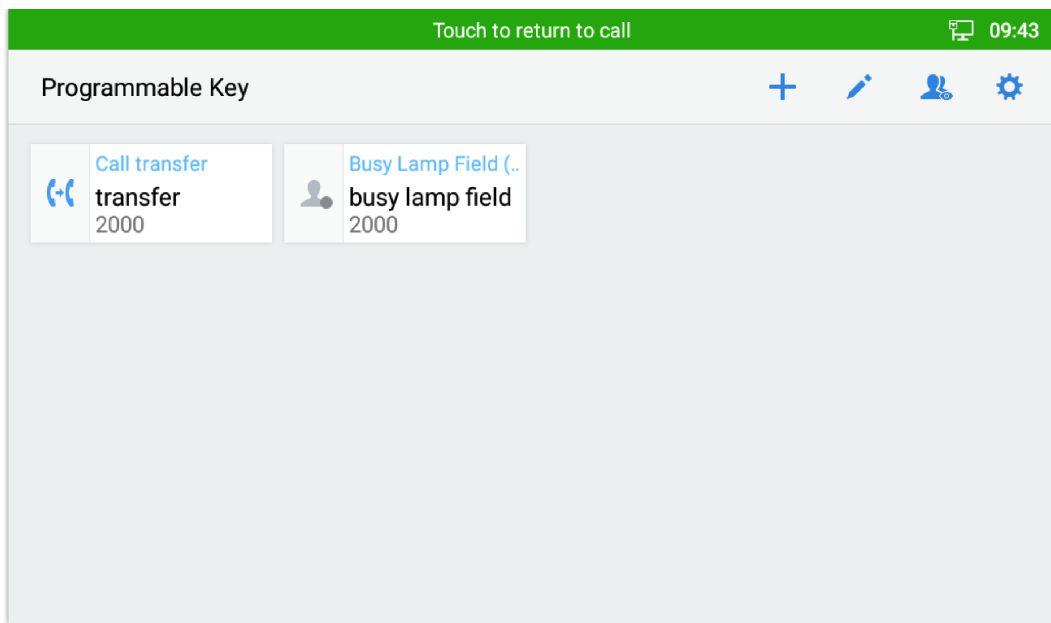
Figure 70 MPK list
