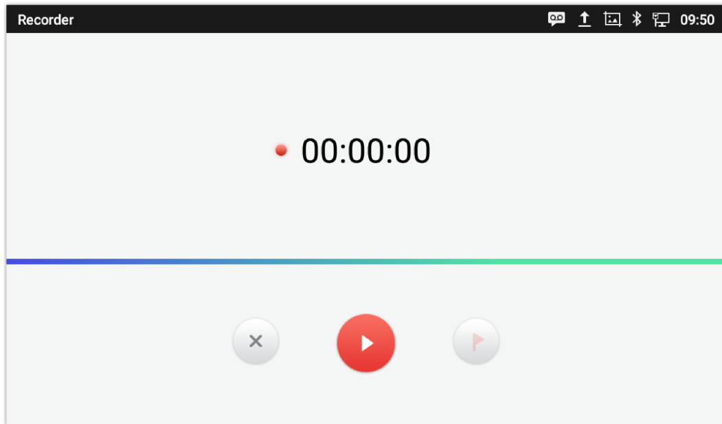
Figure 140 Recording Audio
