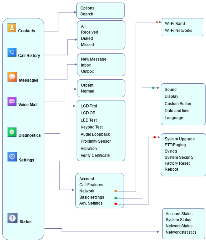
Menu Structure
